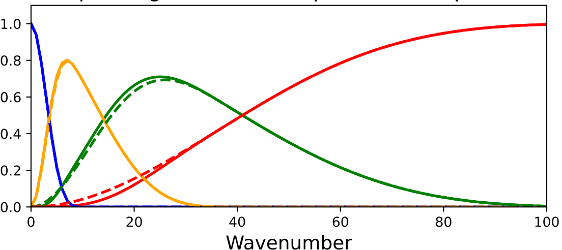
Corresponding recursive and parallel band-pass filters
