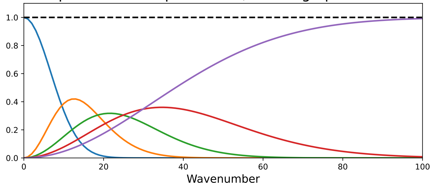
Equivalent band-pass filters, from high-pass filters
