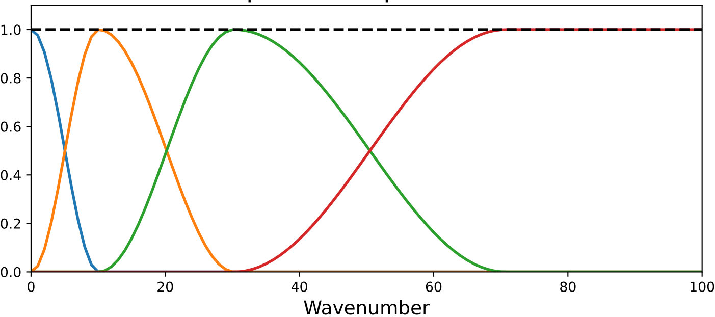
Explicit band-pass filters
