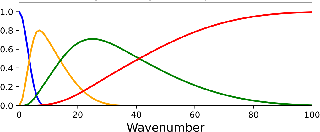
Corresponding band-pass filters
