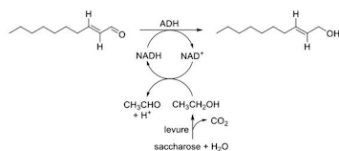
Figure 1: Reaction pathway for the enzymatic reduction of ( E )-2-decenal to the corresponding alcohol via yeast alcohol dehydrogenase (ADH) [3].
