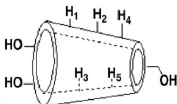
Figure 10: Structure of \beta -cyclodextrin illustrating the internal cavity protons (H3, H5) directly involved in host-guest interactions [7].
