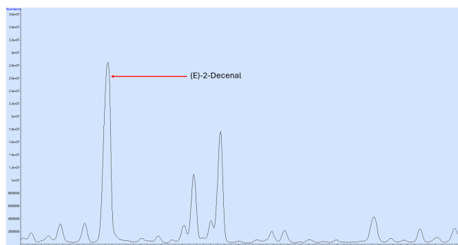
Figure 5: GC-MS chromatogram of the volatile profile from fresh coriander leaves, highlighting the major peak corresponding to ( E )-2-decenal.
