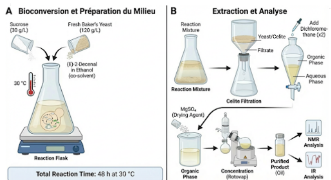
Figure 2: Experimental setup and downstream extraction protocol for the whole-cell bioconversion using S. cerevisiae .
