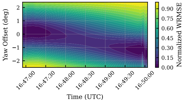
Normalized WRMSE Distribution (Orientation Index: 200)
