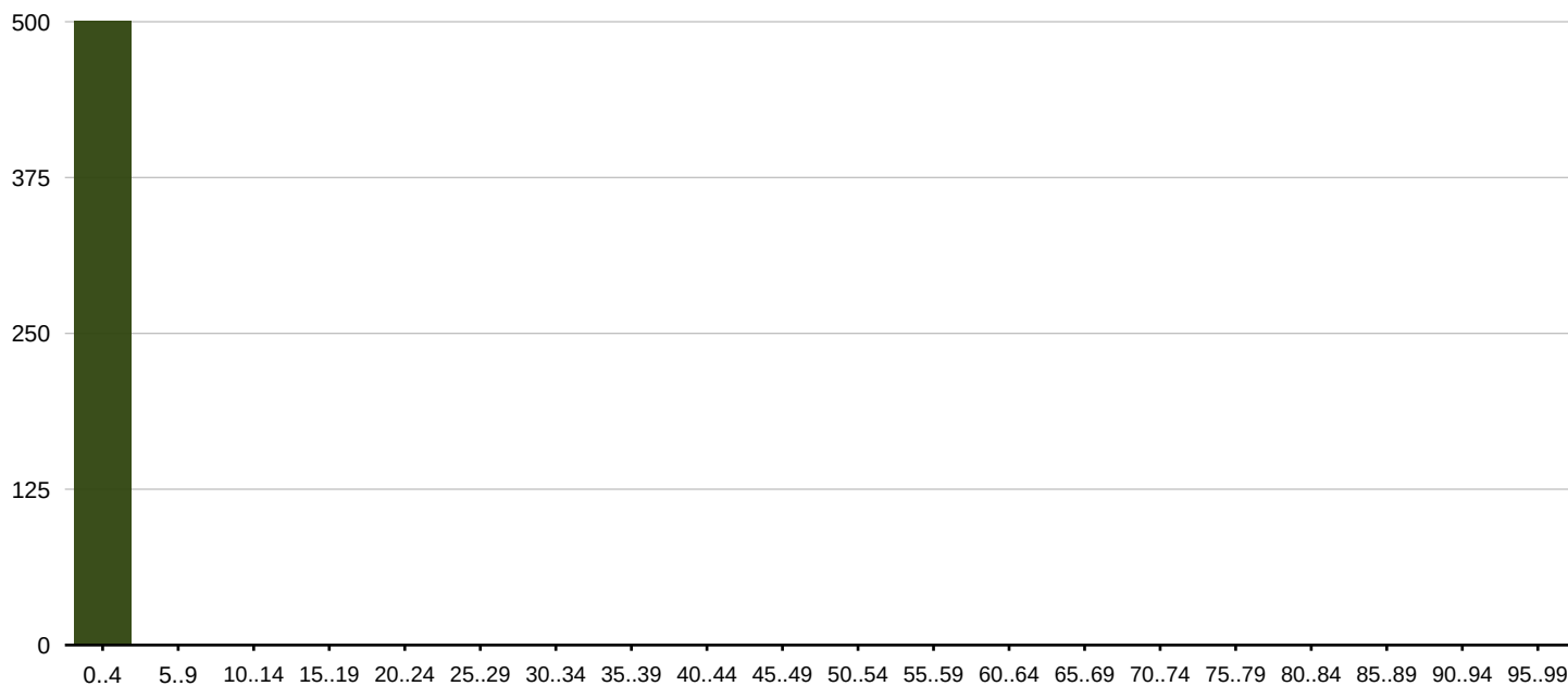
Distribution of final value of Troubled_child_status in 501 randomtest runs
