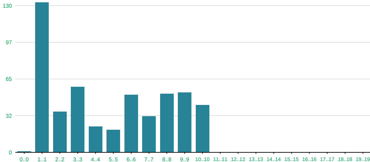
Distribution of final value of Ev_undergraduate_awards in 501 randomtest runs
