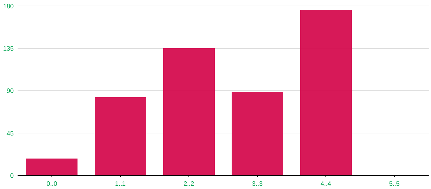
Distribution of final value of Larceny in 501 randomtest runs
