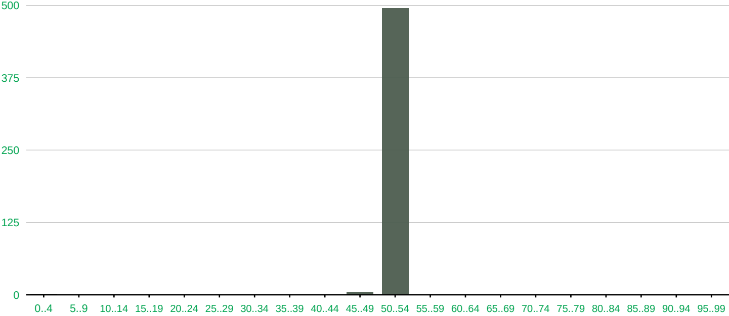
Distribution of final value of Troubled_child_like in 501 randomtest runs
