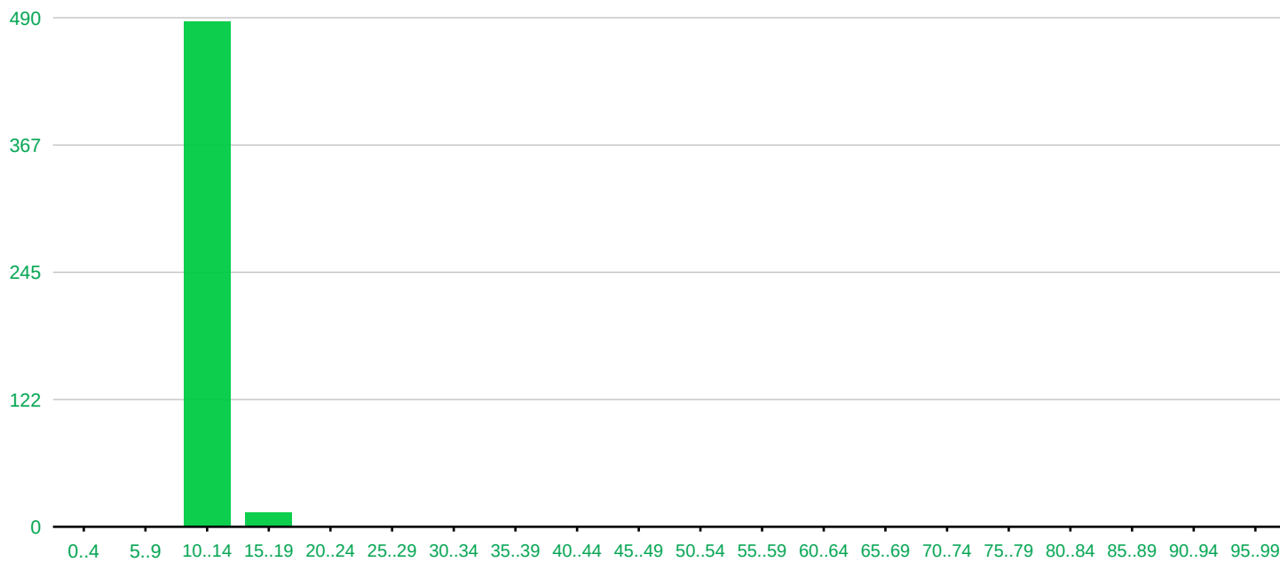
Distribution of final value of D_greed in 501 randomtest runs
