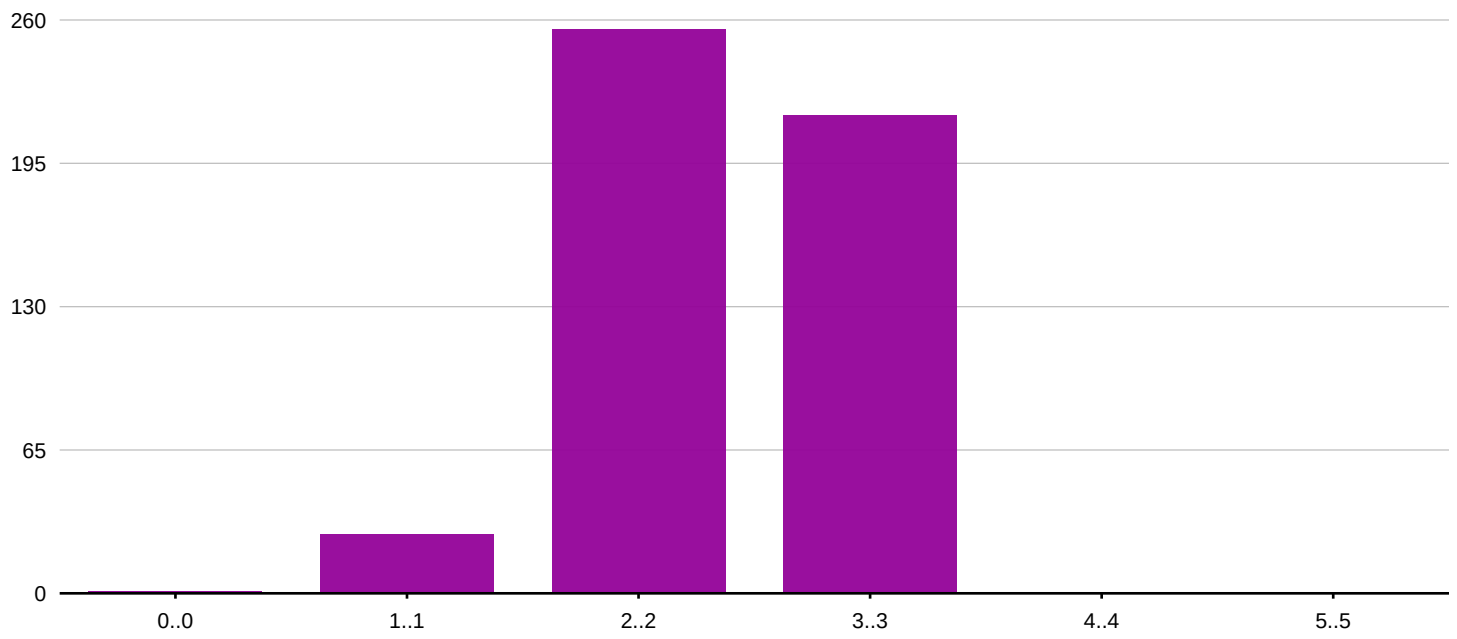
Distribution of final value of Intelligence in 501 randomtest runs
