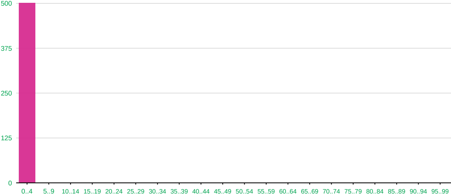
Distribution of final value of Lior_romance in 501 randomtest runs
