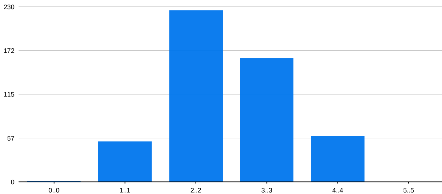
Distribution of final value of Wits in 501 randomtest runs
