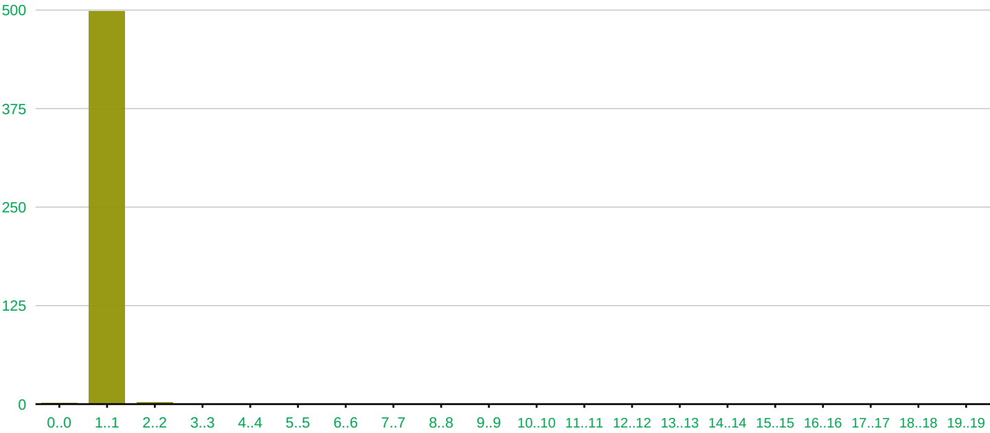
Distribution of final value of Ev_ch1_owen_outcome in 501 randomtest runs
