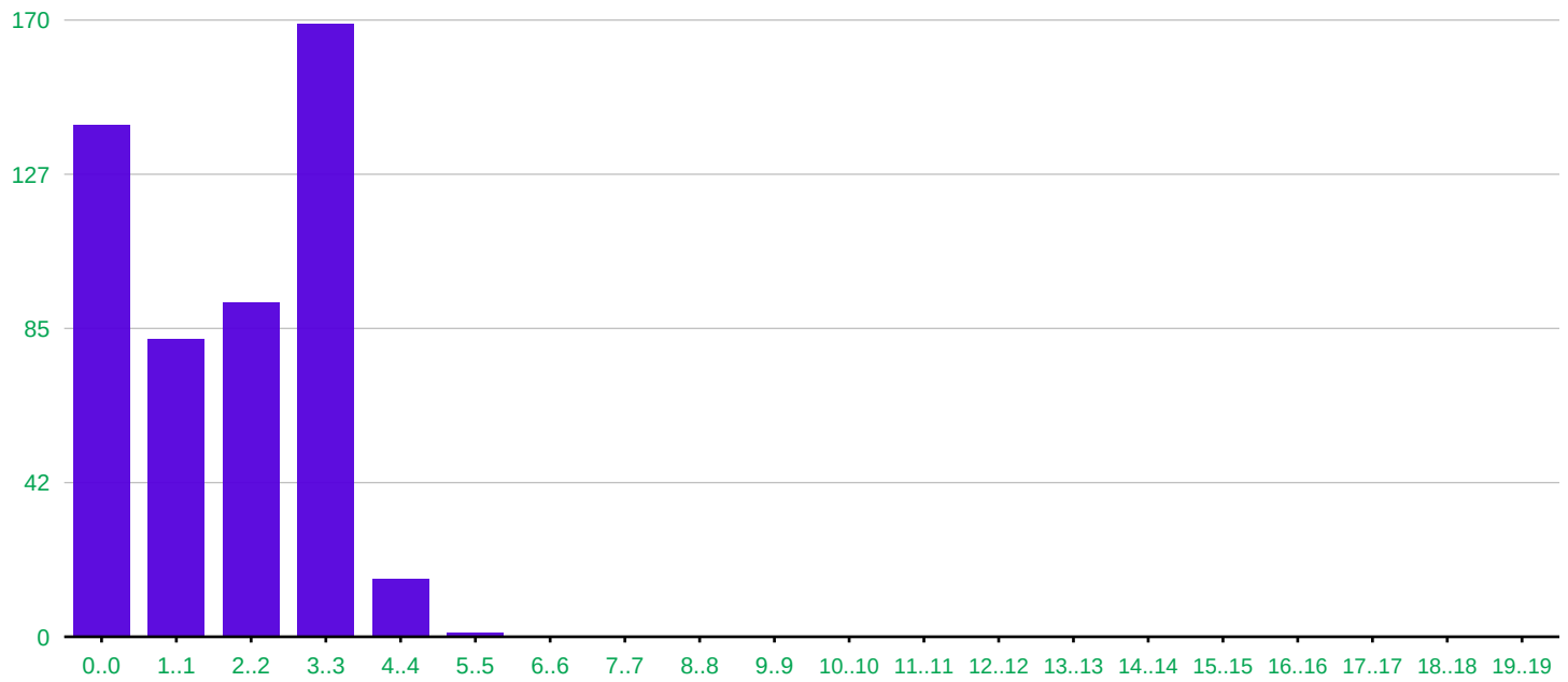
Distribution of final value of Pc_spfc_wounds in 501 randomtest runs
