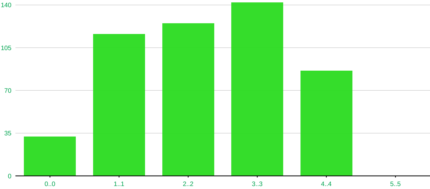
Distribution of final value of Persuasion in 501 randomtest runs
