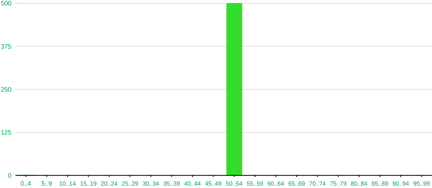
Distribution of final value of The_journo_like in 501 randomtest runs
