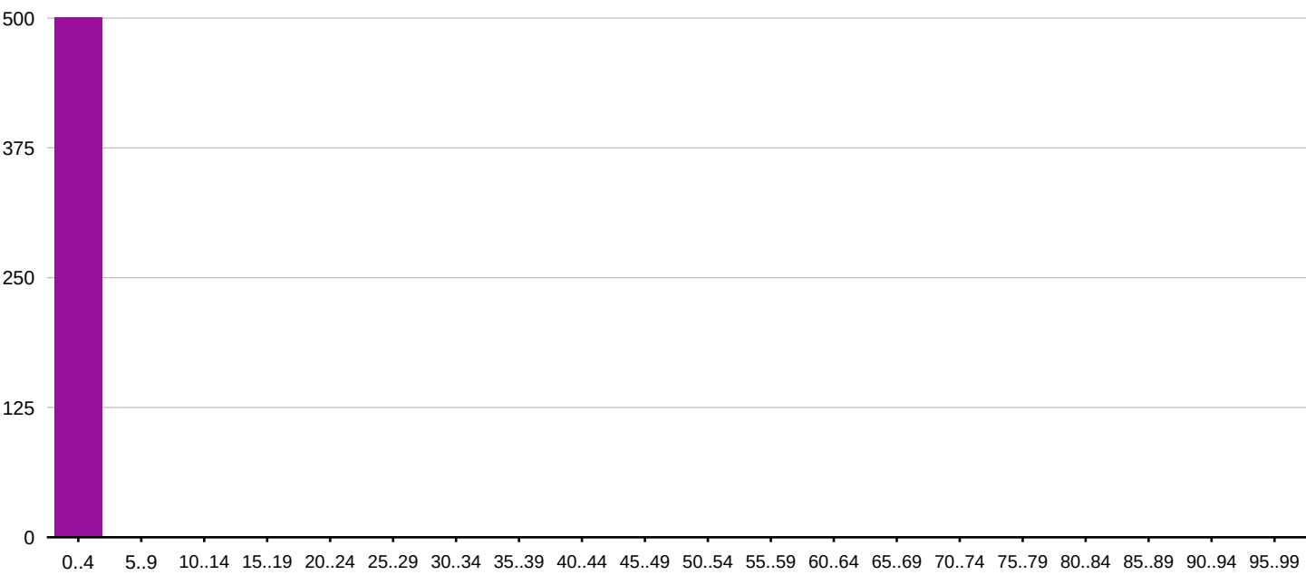
Distribution of final value of Camarilla_leverage in 501 randomtest runs
