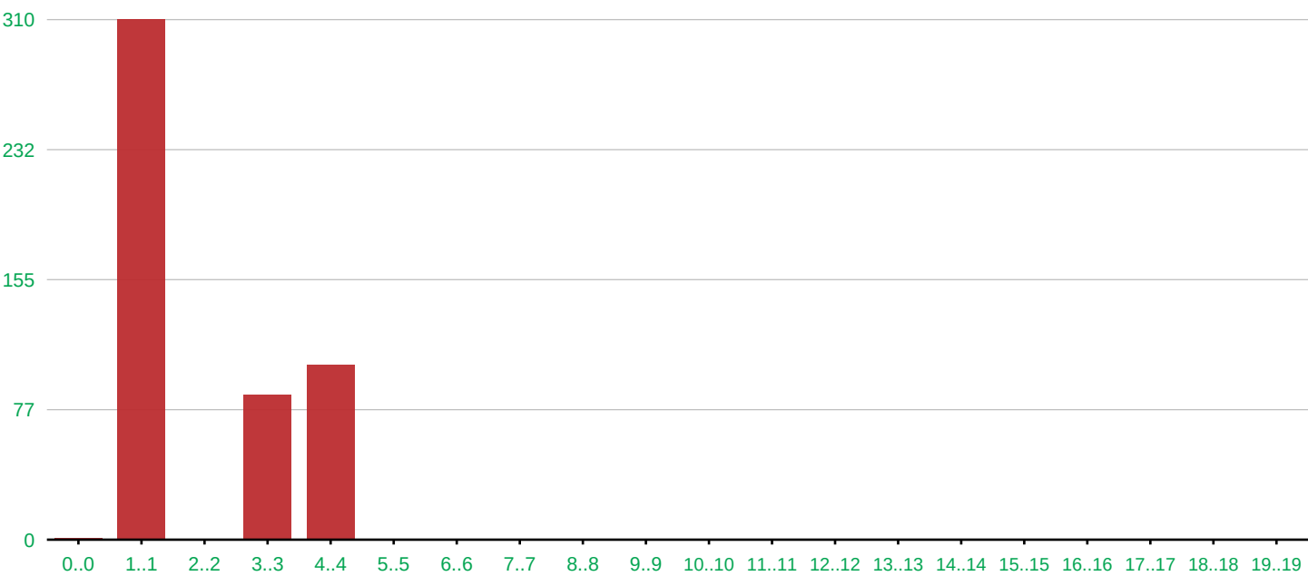
Distribution of final value of Ev_ch1_bitten_by_owen in 501 randomtest runs
