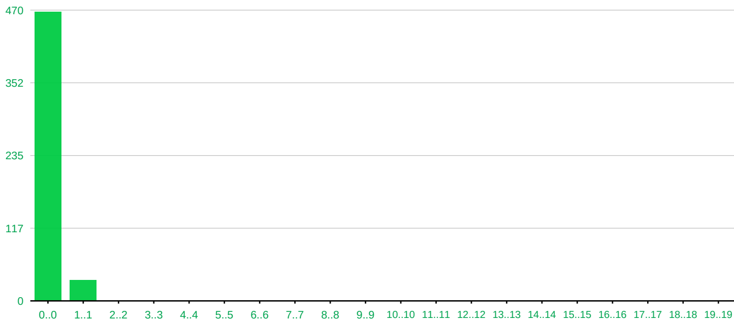
Distribution of final value of Ev_ch1_clue_outfit in 501 randomtest runs
