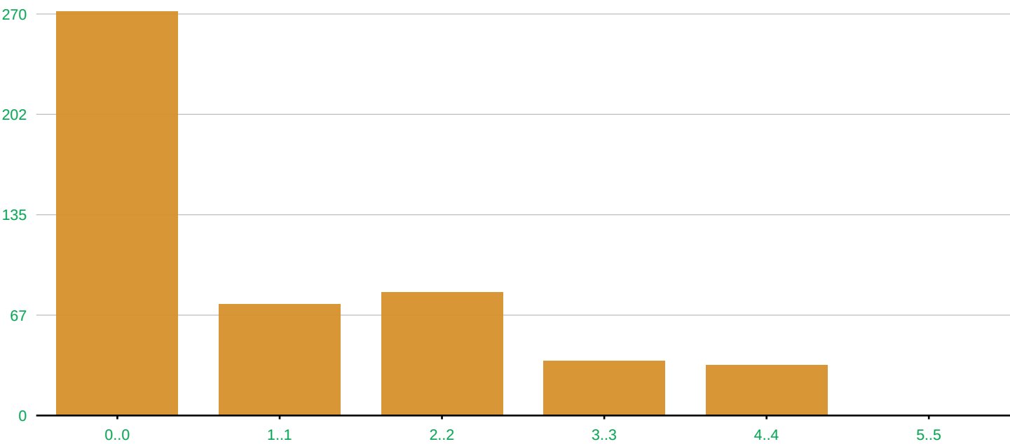
Distribution of final value of Animal_ken in 501 randomtest runs
