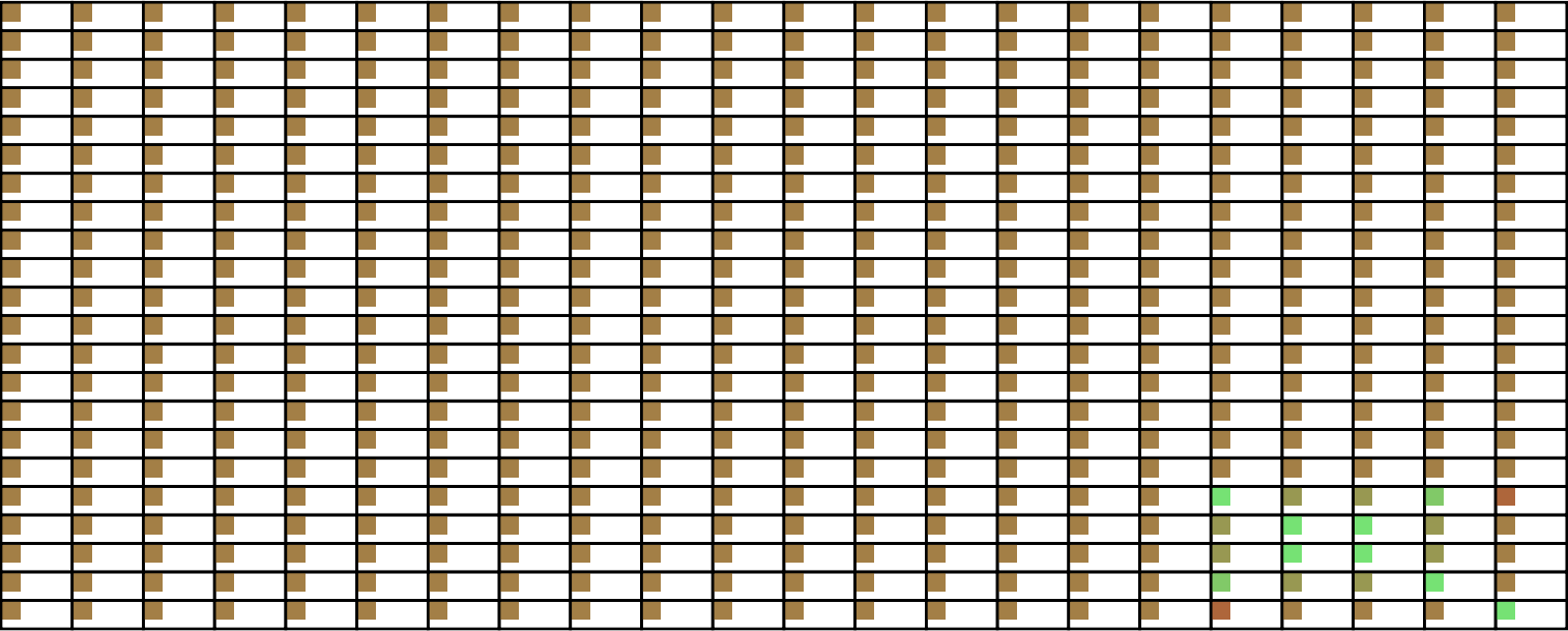
Pearson's correlation coefficient for pairs of secondaries stats
