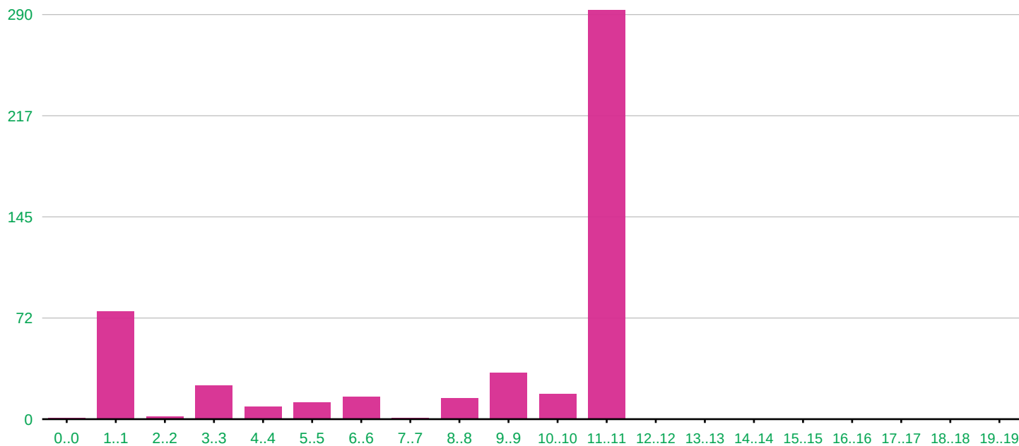
Distribution of final value of Ev_ch1_owen_foyer_clash in 501 randomtest runs
