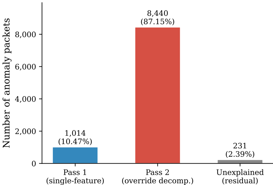
CF pass distribution (n=9,685 anomalies)
