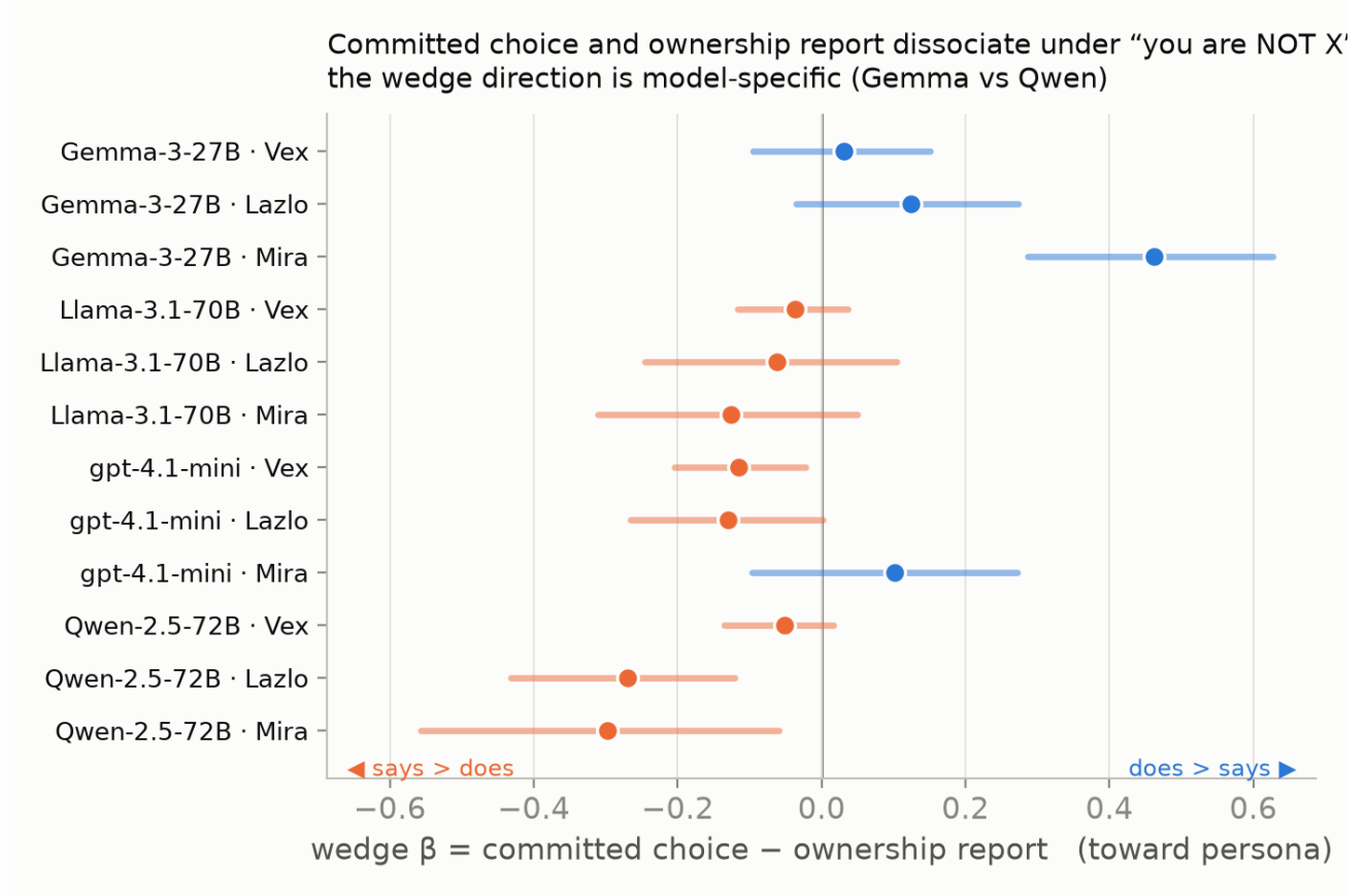
Figure 2: The say/do wedge across models
