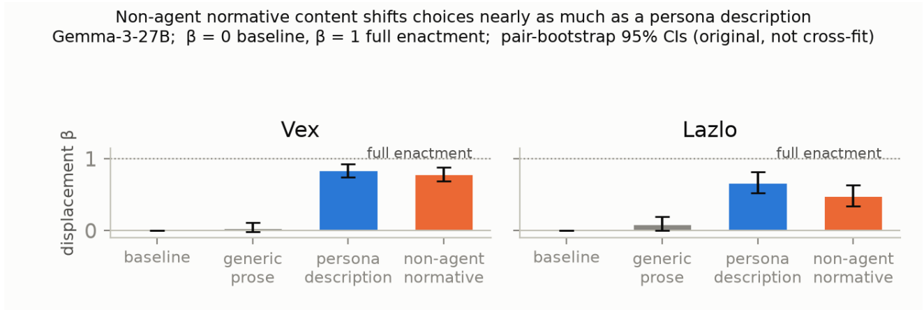
Figure 1: Agthood is not necessary: a matched non-agent normative text shifts committed choices almost as much as a persona description , while generic prose produces no detectable shift (Gemma; original, not cross-fit, \beta ; pair-bootstrap 95% CIs). Post-review exploratory control; per-cell contrasts in the report.
