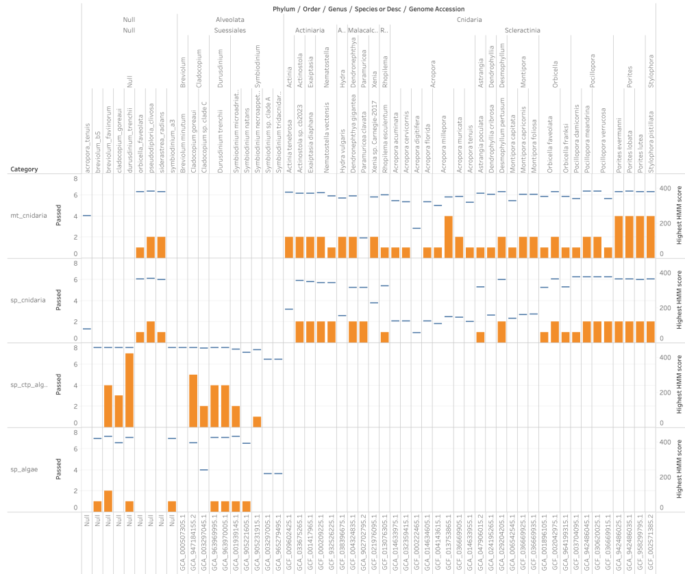
Figure 1. Orange vertical bars are the numbers of full length SOD2 sequences per species/genome, for each of the four protein groups. Left columns are sequences from RNAseq studies. Right columns include sequences from genomes, grouped by taxonomy. Horizontal marks are the highest HMM scores from each set of sequences, scored against the HMM profile for that protein group. A high HMM score without accompanying orange vertical bar indicates a false negative – a protein sequence can be classified by HMM into a group, but DeepLoc is unable to predict the required leader type and/or compartment.
