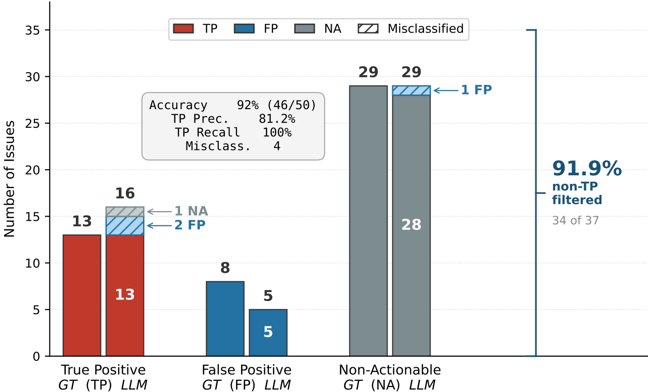
Ground Truth vs. LLM Classifier (9-Tool + Prompt Caching, Claude Sonnet 4.5, n = 50, Pilot 1)
