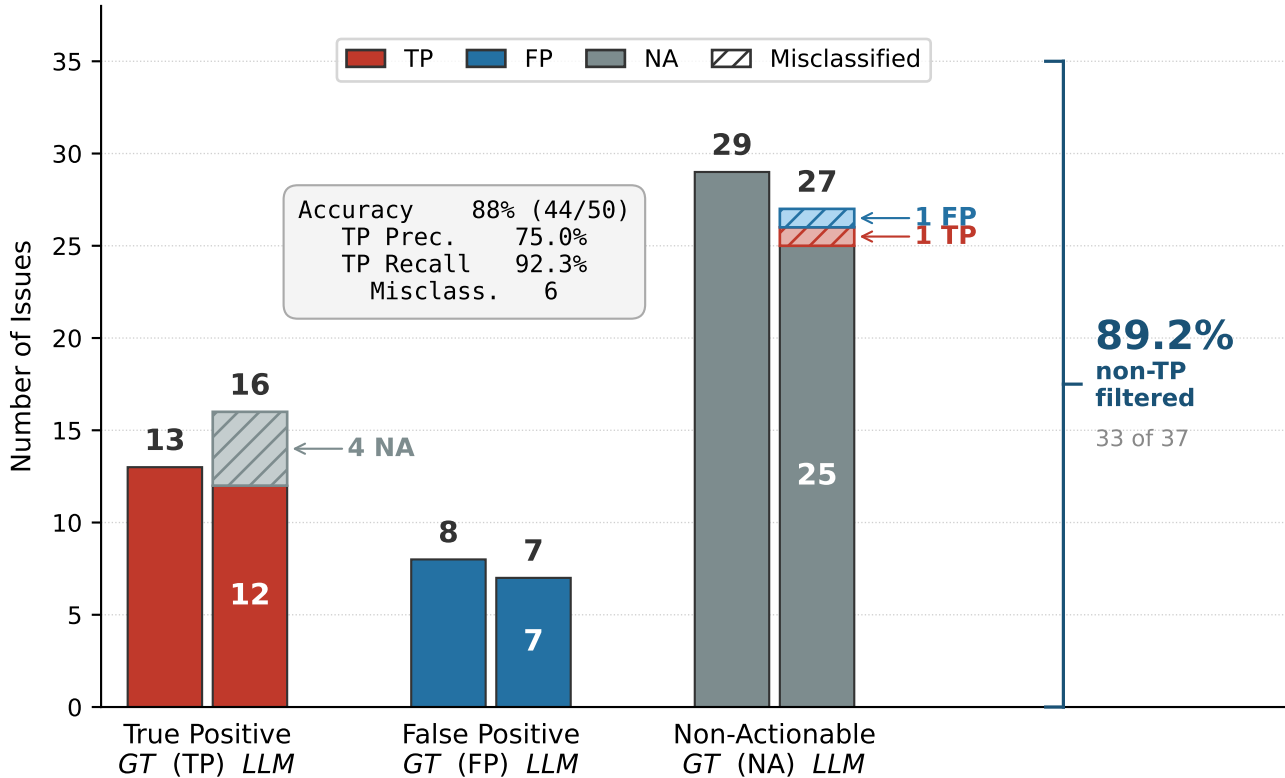
Ground Truth vs. LLM Classifier (9-Tool + SEARCH Cap, Claude Sonnet 4.5, n = 50, Pilot 1)
