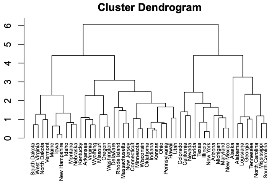
Figura 12.7: US Arrest Hierarchical Clustering, retomado de Chang (2020, p 216) [Cha20]
