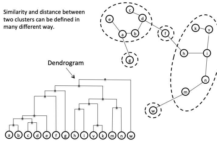
Figura 12.9: Agglomerative Clustering Algorithm and Dendrogram, retomado de Chang (2020, p 219) [Cha20]
