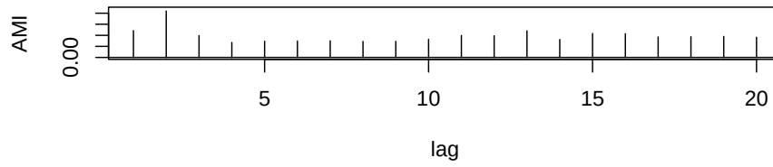
Average Mutual Information of D_flu
