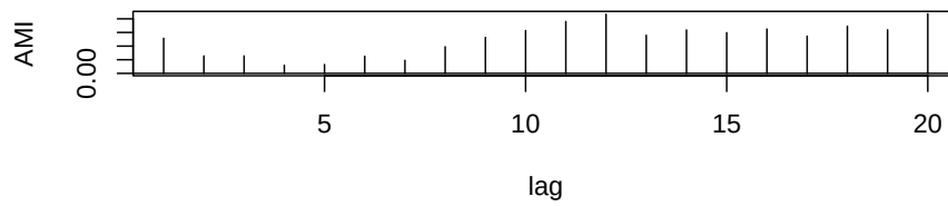
Average Mutual Information of residuals
