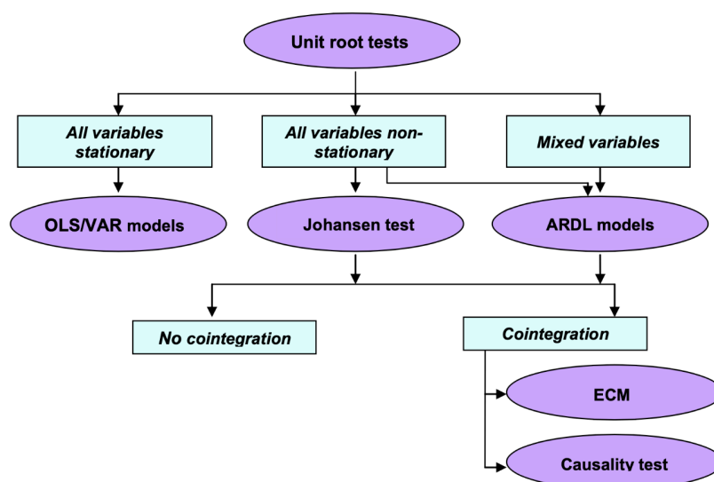
Figura 5.13: Method selection for time series data. OLS: Ordinary least squares; VAR: Vector autoregressive; ARDL: Autoregressive distributed lags; ECM: Error correction models, retomado de: Shrestha y Bhatta [-@shresthabhatta2018]
