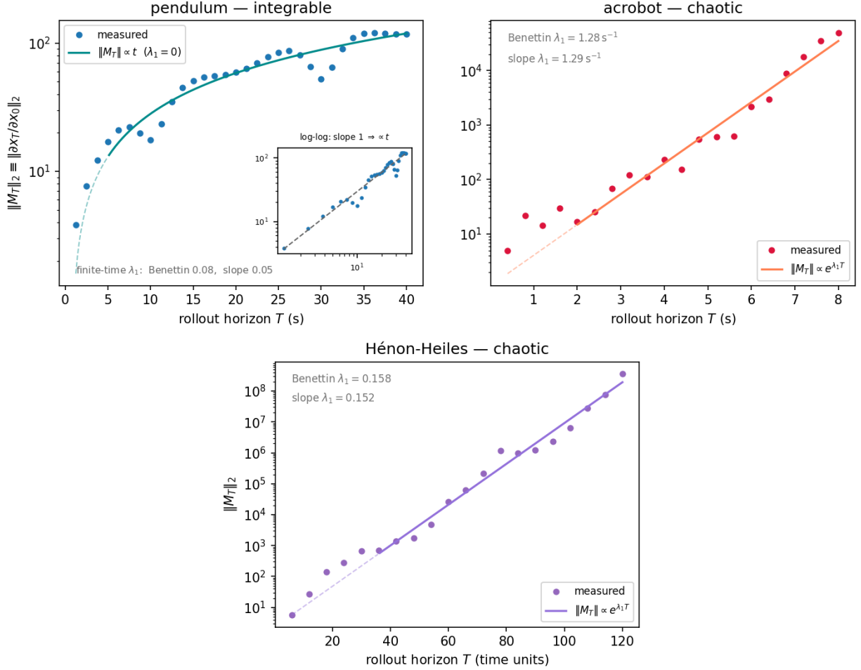
Figure 1: Gradient gain \|\partial x_T / \partial x_0\|_2 versus rollout horizon T (semilog), each panel over its own time window. Top-left, integrable pendulum: linear growth \|M_T\|_2 \propto T with \lambda_1 = 0 (inset: log-log slope 1); the quoted finite-time \lambda_1 are window artifacts that decay to 0. Top-right, chaotic acrobot: exponential growth, log-slope 1.29 \text{ s}^{-1} matching the same-orbit Benettin \lambda_1 = 1.28 \text{ s}^{-1} . Bottom, chaotic Hénon–Heiles: likewise exponential at a smaller rate, log-slope 0.152 against Benettin 0.158 (dimensionless units). Fits are taken past the initial transient (solid; dashed extrapolation).
