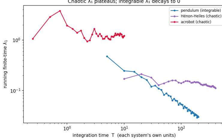
Figure 2: Running finite-time \lambda_1 (Benettin) versus integration time. The chaotic acrobot and Hénon–Heiles settle onto positive plateaus; the integrable pendulum decays toward zero as \ln T/T . This plateau-versus-decay separates Hénon–Heiles’s small but genuine \lambda_1 from the pendulum’s finite-time floor, independently of magnitude.
