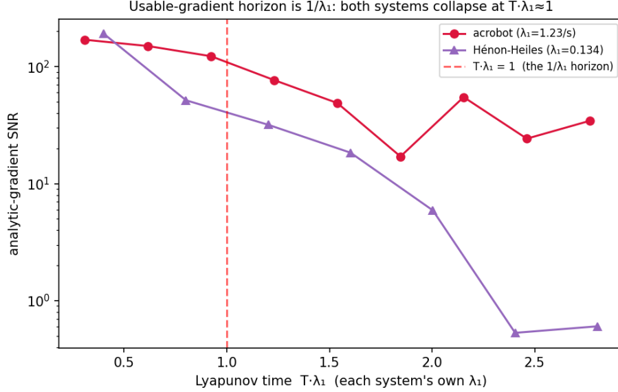
Figure 4: Analytic-gradient SNR versus Lyapunov time T\lambda_1 for two chaotic systems whose \lambda_1 differ tenfold (acrobot 1.23\text{ s}^{-1} , Hénon–Heiles 0.13 ), each on its own \lambda_1 . Both collapse at the same T\lambda_1 \approx 1 (dashed): the gradient’s direction decorrelates across nearby initial conditions even as its magnitude keeps growing, so the usable-gradient horizon is 1/\lambda_1 —set by the Lyapunov clock, not the rollout length.
