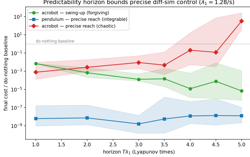
Figure 4: Optimisation through the differentiable simulator on the chaotic acrobat versus rollout horizon T\lambda_1 . Normalized final cost (achieved cost / do-nothing baseline; geometric mean over reach targets, shaded 10–90% band). A forgiving objective (swing the hand up; green) and the integrable pendulum’s precise target-reaching (blue) stay orders of magnitude below the do-nothing baseline (dotted) at every horizon, while the chaotic acrobat’s precise target-reaching (red) rises through the baseline near the predictability horizon T\lambda_1 \approx 4.6 ( 1/\lambda_1 up to the logarithmic factor of Section 4.3) and blows up beyond it as the e^{2\lambda_1 T} gradient gain makes the descent diverge; the widening red band marks the loss of reliability. The horizon bounds precise differentiable-sim control; forgiving objectives and integrable dynamics show no wall.
