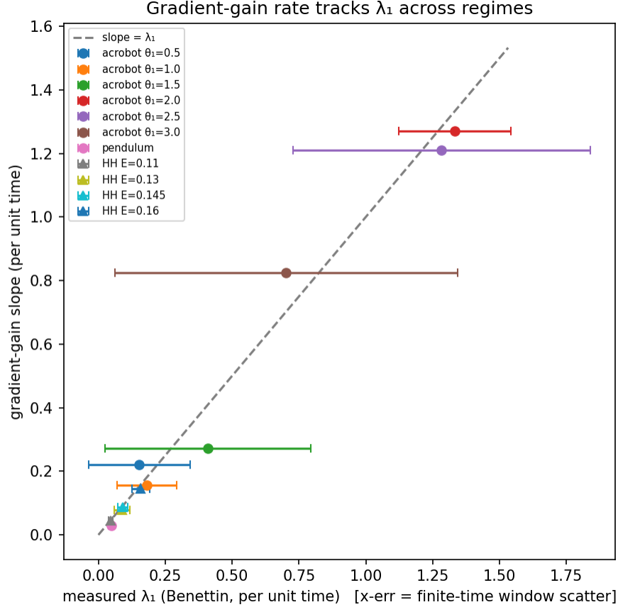
Figure 2: Gradient-gain slope versus Benettin \lambda_1 across an acrobot energy sweep ( \theta_1 = 0.5 \rightarrow 3.0 ), the pendulum, and a Hénon–Heiles energy sweep (a second, independent chaotic system; triangles); all cluster on y = x (correlation 0.99). Units are each system’s own inverse time (mechanical systems in s^{-1} , Hénon–Heiles dimensionless), so y = x is the unit-free statement slope = \lambda_1 . Horizontal bars are finite-time Lyapunov window scatter.
