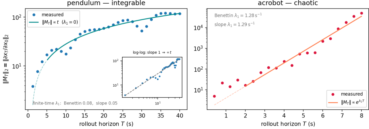
Figure 1: Gradient gain \|\partial x_T / \partial x_0\|_2 versus rollout horizon T in seconds (semilog), each panel over its own physical-time window. Integrable pendulum (left): linear growth \|M_T\|_2 \propto T with \lambda_1 = 0 (inset: log-log slope 1); the quoted finite-time \lambda_1 are window artifacts that decay to 0. Chaotic acrobot (right): exponential growth, log-slope 1.29 \text{ s}^{-1} matching the same-orbit Benettin \lambda_1 = 1.28 \text{ s}^{-1} . Fits are taken past the initial transient (solid; dashed extrapolation).
