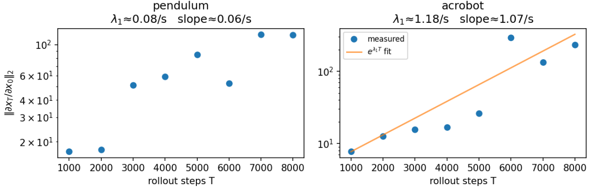
Figure 1: Gradient gain \|\partial x_T / \partial x_0\|_2 versus rollout horizon T (semilog). Integrable pendulum (left): sub-exponential, \lambda_1 \approx 0 . Chaotic acrobot (right): exponential growth whose log-slope ( 1.07 \text{ s}^{-1} ) matches the Benettin \lambda_1 ( 1.18 \text{ s}^{-1} ).
