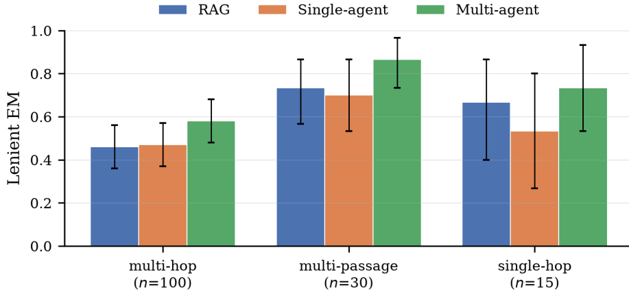
Figure 2: L-EM by stratum and architecture, unconstrained mode. Error bars are bootstrap 95% CIs. The unanswerable stratum ( n=8 ) is omitted because answer metrics are 0 there by definition.
