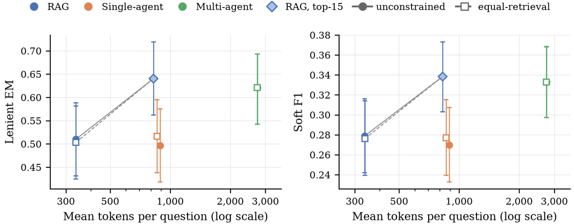
Figure 2: Quality versus mean tokens per question (log scale) with bootstrap 95% CIs. Filled circles: unconstrained; open squares: equal-retrieval; diamonds: RAG top-15 (one run, included in both frontiers). Lines connect Pareto-optimal systems (solid: unconstrained; dashed: equal-retrieval). The two multi-agent points almost coincide.
