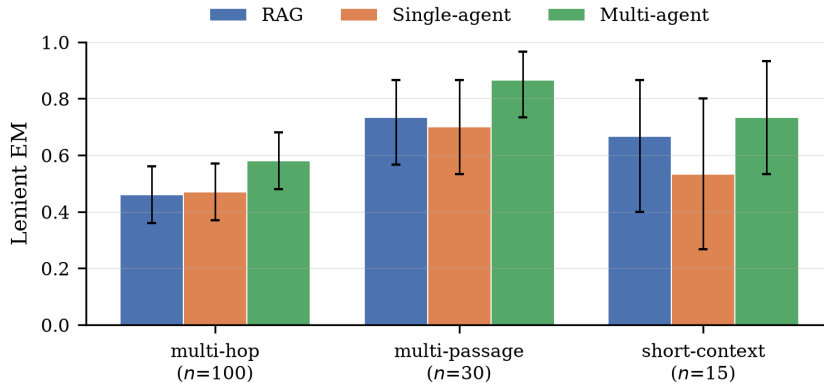
Figure 1: L-EM by stratum, unconstrained mode, with bootstrap 95% CIs (RAG top-5).
