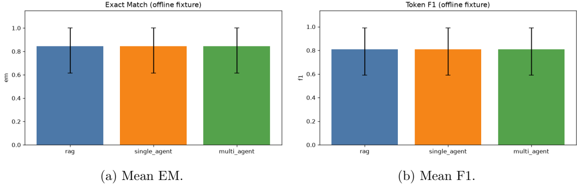
Figure 2: Offline-fixture answer metrics by architecture. Bars are essentially identical; the evaluation signal for this run is efficiency, not quality separation.
