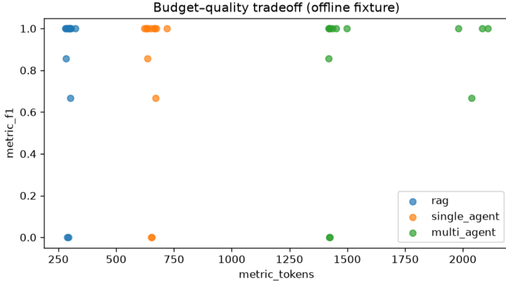
Figure 1: Budget-quality tradeoff on the offline fixture (per-example F1 vs. tokens). Architectures share similar F1 mass near 1.0 with a common failure at F1=0; multi-agent occupies a higher token regime. This plot illustrates process overhead under matched heuristic quality—not a live LLM ranking.
