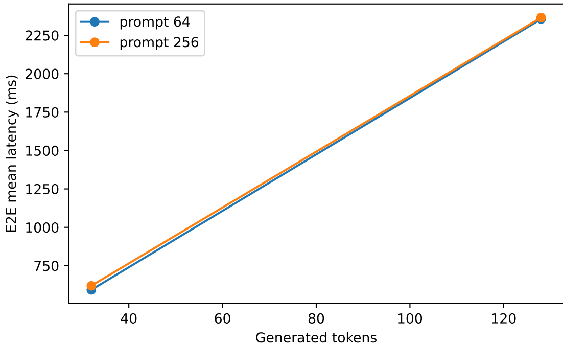
Latency vs generation length (bf16, eager, batch 1)
