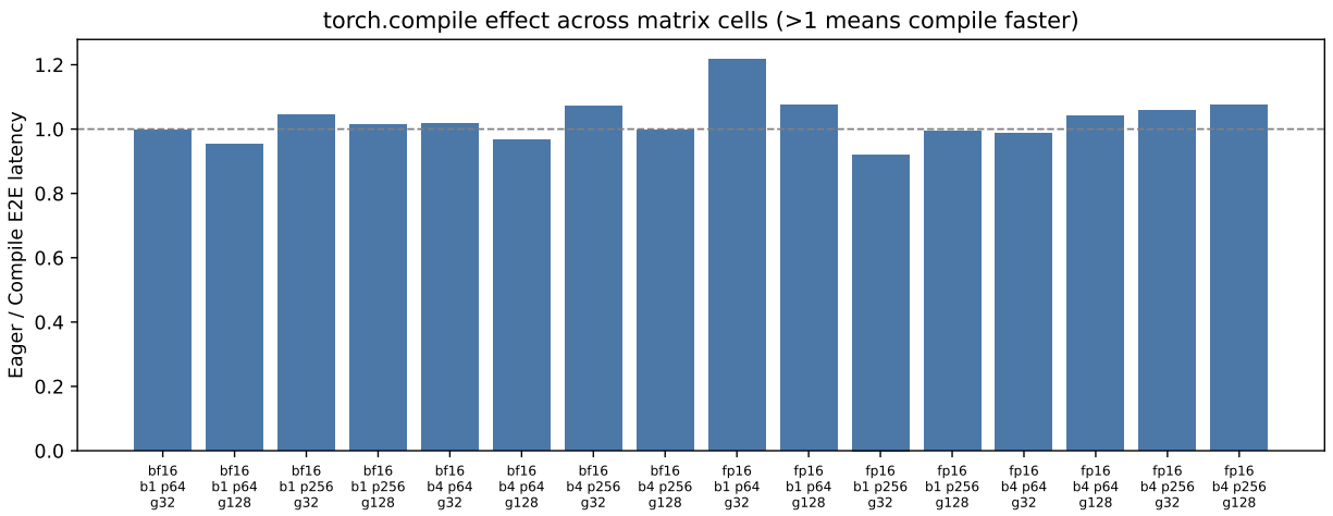
Figure 4: Eager/compile end-to-end latency ratios (> 1 means compile is faster).
