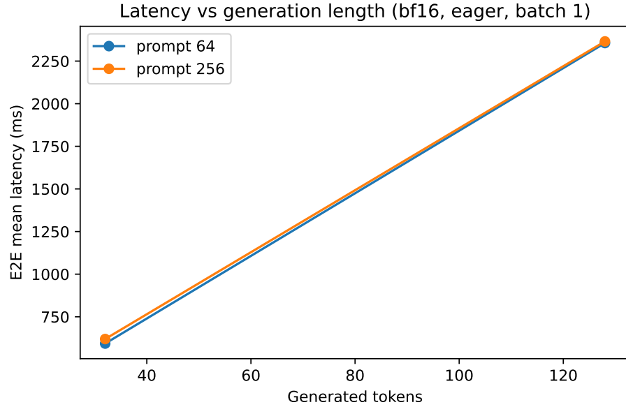
Figure 3: Latency versus generation length (BF16, eager, batch 1).
