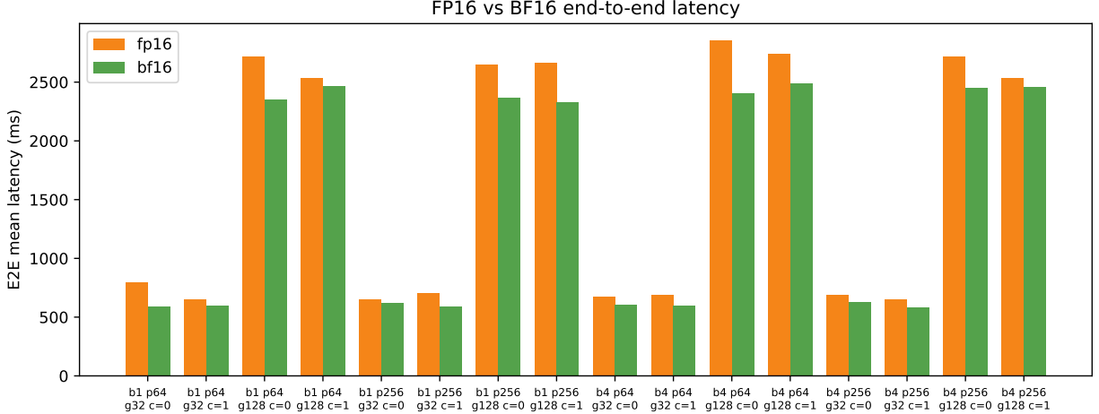
Figure 1: End-to-end mean latency for FP16 vs. BF16 across matched matrix cells.
