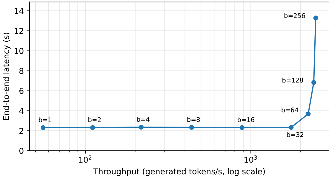
Batch-size sweep: BF16, eager, prompt 256, 128 new tokens
