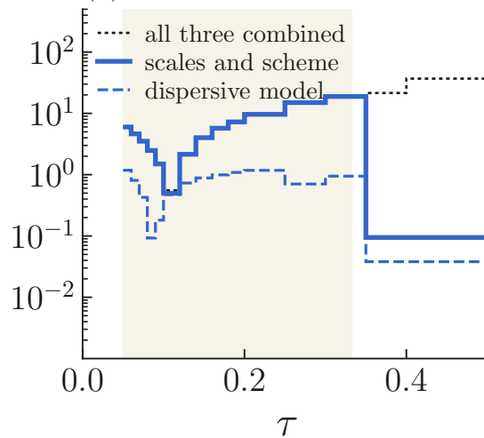
(c) theory
