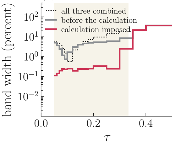
(b) generator
