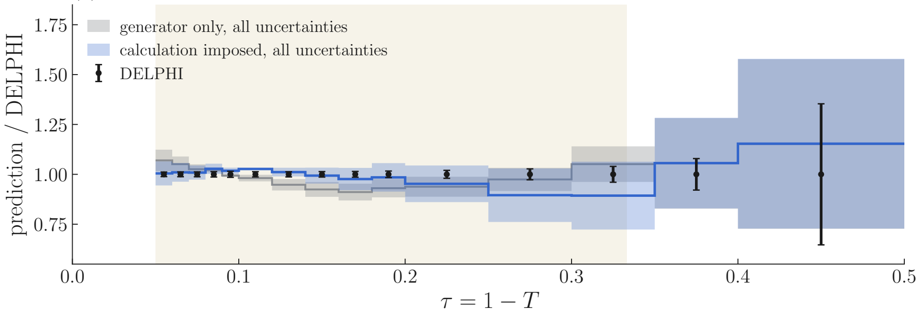
(a) generator, theory and learning uncertainties combined
