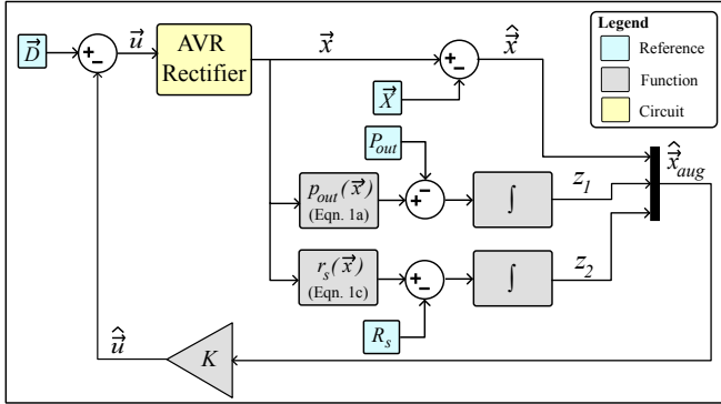
Fig. 5: Block diagram of the state-space control loop. p_{out}(\vec{x}) and r_s(\vec{x}) are given by Eqns. 1a and 1c. \hat{D} contains nominal duties of the buck and boost converters.
