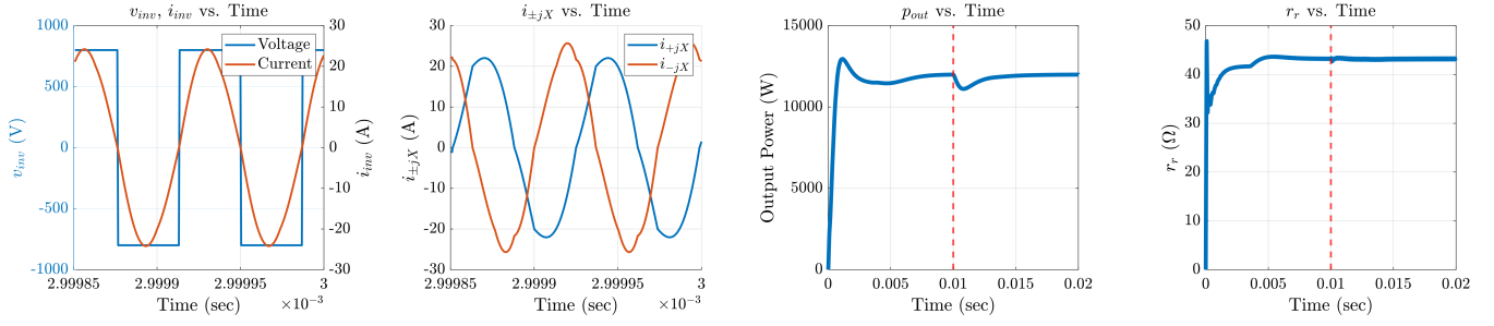
Fig. 4: From left to right: inverter output waveforms v_{inv} and i_{inv} in steady-state; AVR branch currents i_{+jX} and i_{-jX} in steady-state; p_{out} and r_r vs. time, showing the AVR rectifier's startup transient under the proposed controller for t \in [0, 0.01) , followed by a step change in coupling reactance \Delta X_s at time t = 0.01 , marked by the red vertical line.
