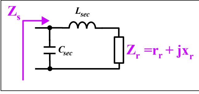
Fig. 6: Schematic illustrating z_s equivalent circuit.
