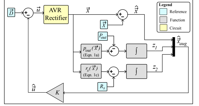
Fig. 4: Block diagram of the state-space control loop. p_{out}(\vec{x}) and r_s(\vec{x}) are given by Eqns. 1a and 1c. \vec{D} contains nominal duties of the buck and boost converters.
