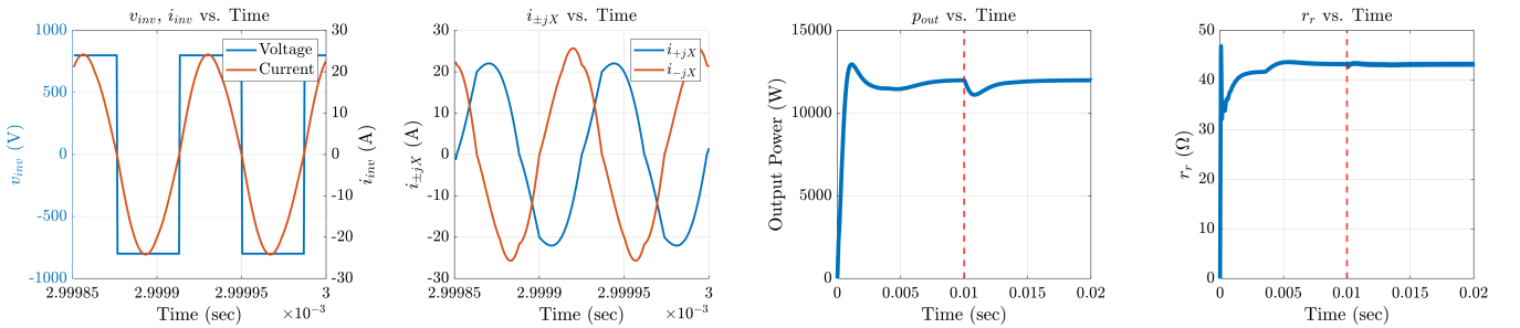
Fig. 5: From left to right: inverter output waveforms v_{inv} and i_{inv} in steady-state; AVR branch currents i_{+jX} and i_{-jX} in steady-state; p_{out} and r_r vs. time, showing the AVR rectifier's startup transient under the proposed controller for t \in [0, 0.01] , followed by a step change in coupling reactance \Delta X_s at time t = 0.01 , marked by the red vertical line.
