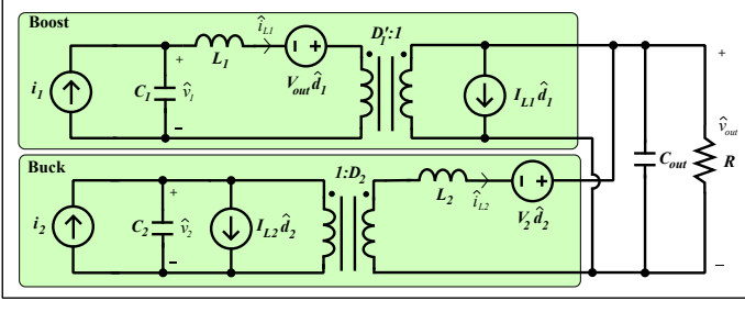
Fig. 3: Schematic of the linearized small-signal model of the AVR rectifier.
