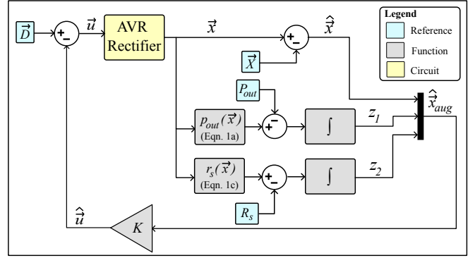
Fig. 4: Block diagram of the state-space control loop. p_{out}(\vec{x}) and r_s(\vec{x}) are given by Eqns. 1a and 1c. \vec{D} contains nominal duties of the buck and boost converters.
