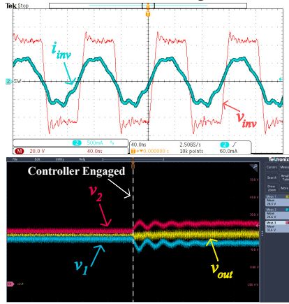
Fig. 7: Top: inverter switch node voltage v_{inv} and current i_{inv} . Bottom: controller activation transient showing v_1 , v_2 , and v_{out} trajectories.
