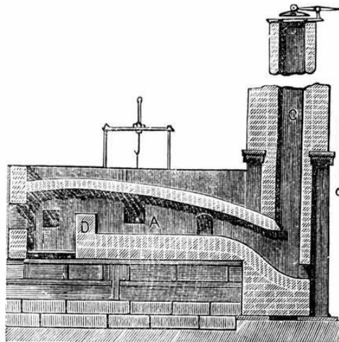
Source S1 : The Puddling Furnace
