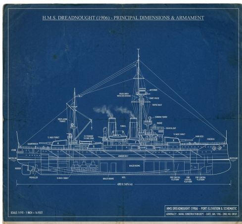
Source A: Official technical blueprint of HMS Dreadnought, 1906.
