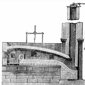
Source B: Patent drawing cross-section of Cort's reverberatory puddling furnace at Funtley.
