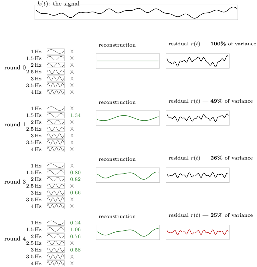
Figure 11: The same story on a real signal: frequencies. Matching pursuit’s native domain. The signal h (top) is decomposed against an overcomplete dictionary of pure tones—the 1–4 Hz band sampled every 0.5 Hz, finer than a 1-second window resolves, so the atoms are redundant and non-orthogonal . Each round grabs the best-matching tone and refits all active magnitudes by least squares—watch 1.5 Hz swing 1.34 \rightarrow 0.80 \rightarrow 1.06 as neighbours enter (the inner loop, and coefficients above 1), while redundant rows (2.5, 3.5, 4 Hz) are left X, never needed. The reconstruction (green) grows to resemble h ’s slow structure, but h also holds fast tones above the band that no atom reaches, so the residual stalls at a necessary 25% of the variance. Overcomplete, redistributing, and leaving real structure behind—the mechanism of the J-lens (push h further out of band and this remainder becomes the majority, as in J-space). Contrast the exact basis of Figure 9.
