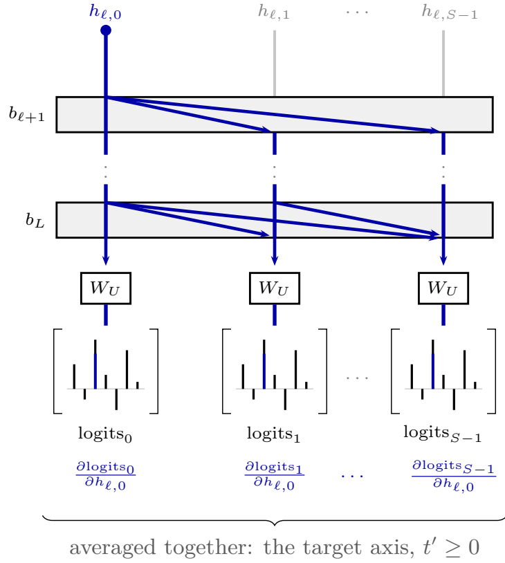
Figure 7: The same pairs, grouped the other way. Figure 6 is oriented toward one logit vector—the causal heads feeding \text{logits}_{S-1} , one panel per source. Here, the dual orientation: one latent, h_{\ell,0} , and every logit vector it touches—its causal tails . Every stream admits the same shared W_U , so the tapped latent’s target axis is this whole fan, one Jacobian per downstream chart (blue bars mark its influence landing). Group the (t, t' \geq t) pairs by target or by source—the set, and the mean the J-lens takes over it, is identical.
