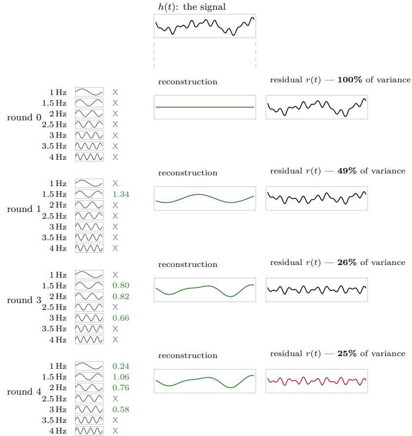
Figure 11: The same story on a real signal: frequencies. Matching pursuit’s native domain. The signal h (top, drawn above the reconstruction column so the two can be compared) is decomposed against an overcomplete dictionary of pure tones—the 1–4 Hz band sampled every 0.5 Hz, finer than a 1-second window resolves, so the atoms are redundant and non-orthogonal . Each round grabs the best-matching tone and refits all active magnitudes by least squares—watch 1.5 Hz swing 1.34 \rightarrow 0.80 \rightarrow 1.06 as neighbours enter (the inner loop, and coefficients above 1), while redundant rows (2.5, 3.5, 4 Hz) are left X , never needed. The reconstruction (green) grows to resemble h ’s slow structure, but h also holds fast tones above the band that no atom reaches, so the residual stalls at a necessary 25% of the variance. Overcomplete, redistributing, and leaving real structure behind—the mechanism of the J-lens (push h further out of band and this remainder becomes the majority, as in J-space). Contrast the exact basis of Figure 9.
