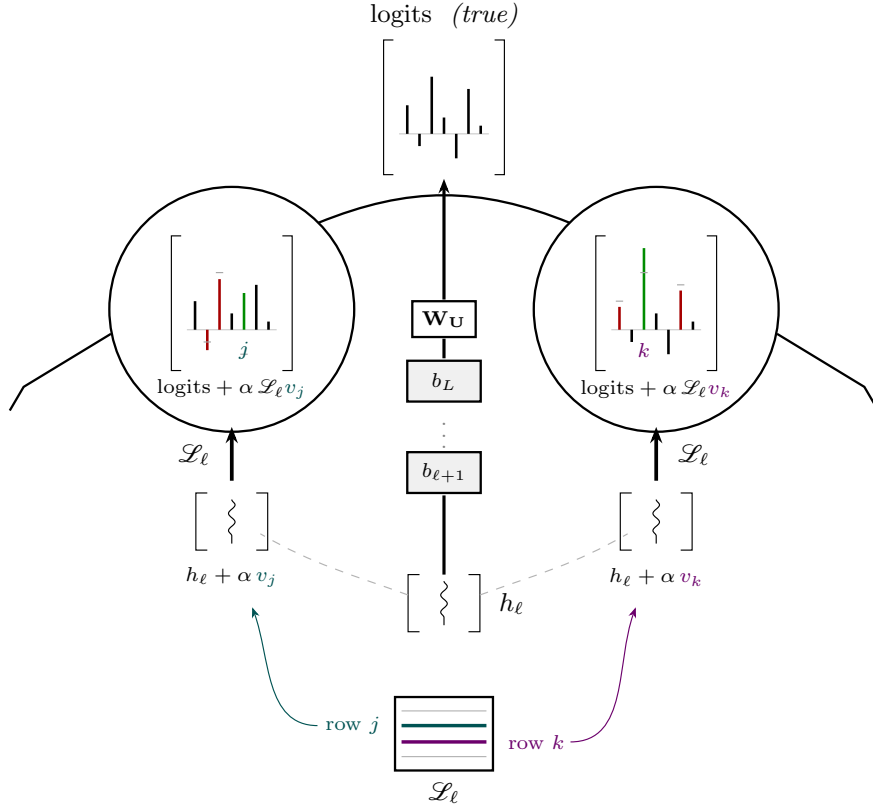
Figure 5: Counterfactual J-vision : without rerunning the network, we can attain approximations of where logits will go with specific nudges on h_\ell . The J-lens enables this vision. The true state h_\ell (center) earns its logits the hard way—up through every remaining block and \mathbf{W}_U . The flanking states are tweaked copies of h_\ell , each nudged along a row of the J-lens \mathcal{L}_\ell itself (rows j and k , drawn out of the matrix at bottom)—and they never run the network at all: through the glass, \Delta \text{logits} = \mathcal{L}_\ell \Delta h , one matrix multiply. Green bars were raised by the tweak, red lowered; gray ticks mark the true heights. Each eye’s tall green bar sits exactly at the token whose row it was steered with.
