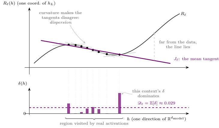
Figure 9: What the lens is: the average of the local linear behaviors J_{\ell}(h) = \frac{\partial h_L}{\partial h} —i.e. the atom \frac{\partial h_{L,t'}}{\partial h_{\ell,t}} at each visited latent h = h_{\ell,t} —across the activations the model actually visits (dots; one gray tangent each). Where R_{\ell} curves within the visited region, the tangents fan—that spread is the dispersion \mathcal{D}_{\ell} = \mathbb{E} \|J_{\ell}(h) - J_{\ell}\|^2 . And the mean tangent is a local instrument: far from the sampled region, the line and the function part ways. The lower panel makes the spread concrete: each bar is one visited latent’s \delta = \|J_{\ell}(h) - J_{\ell}\|^2 —how far its tangent tilts from the mean—and \mathcal{D}_{\ell} is simply their average, pulled up here by the lone high-curvature latent at the region’s right edge.
