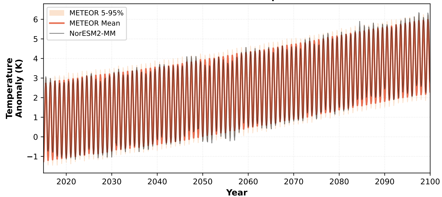
SSP5-8.5 - Global Temperature
