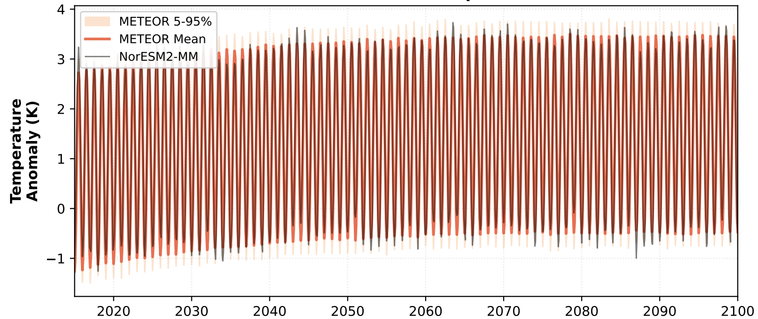
SSP5-8.5 - Global Temperature
