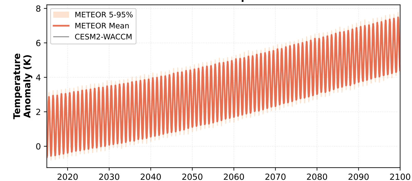
SSP5-8.5 - Temperature
