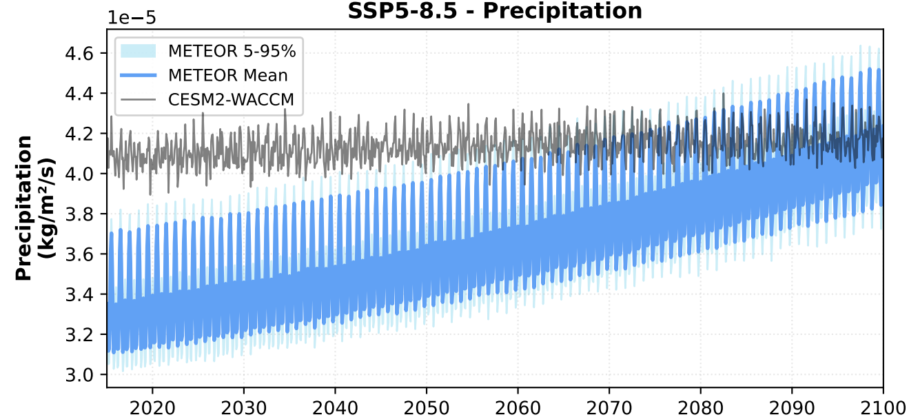
SSP5-8.5 - Precipitation
