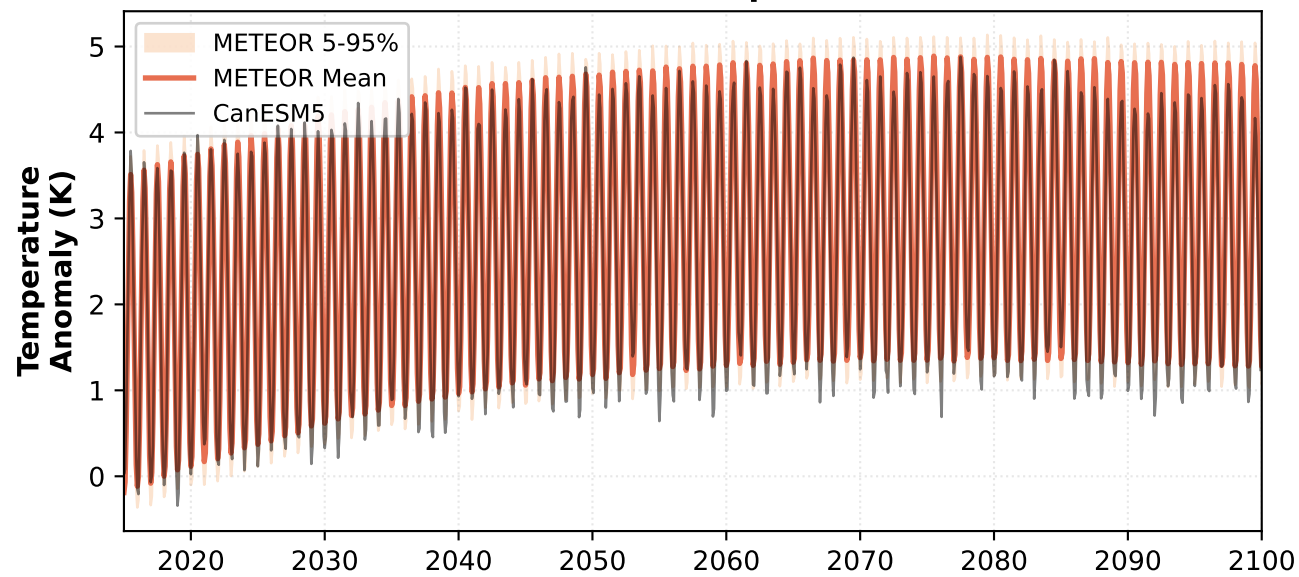
SSP2-4.5 (in-sample) - Temperature
