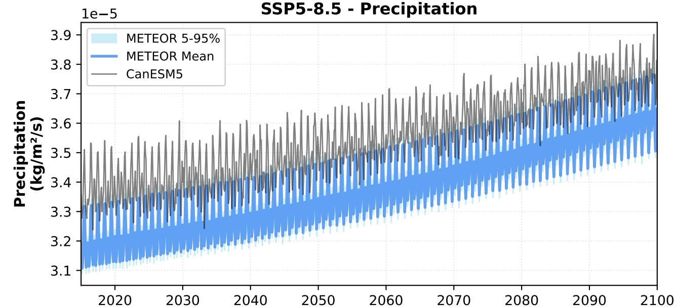
SSP5-8.5 - Precipitation
