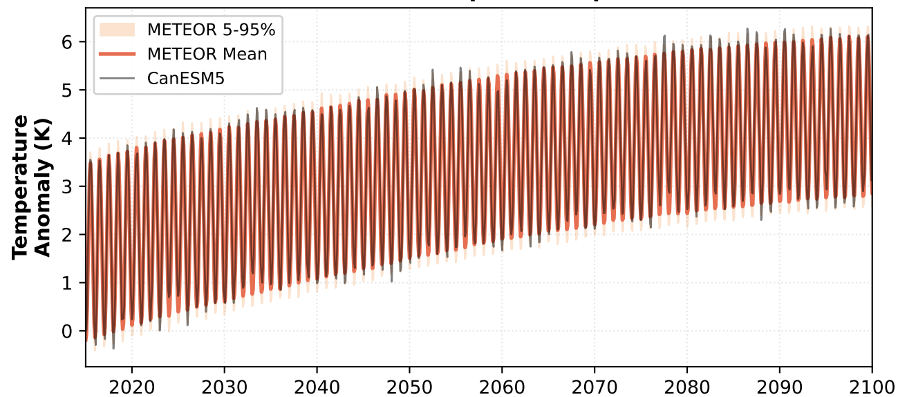
SSP5-8.5 - Temperature
