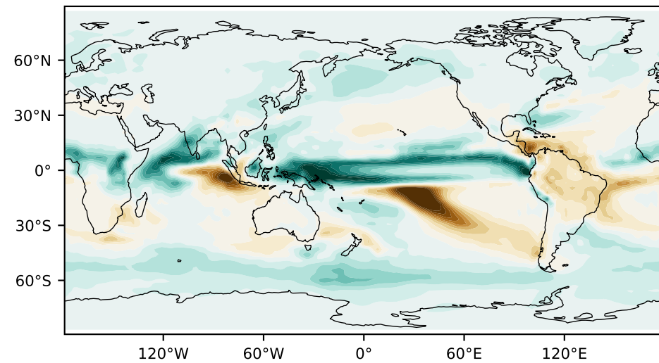
CanESM5
