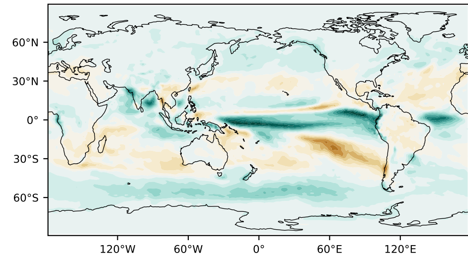
CNRM-ESM2-1
