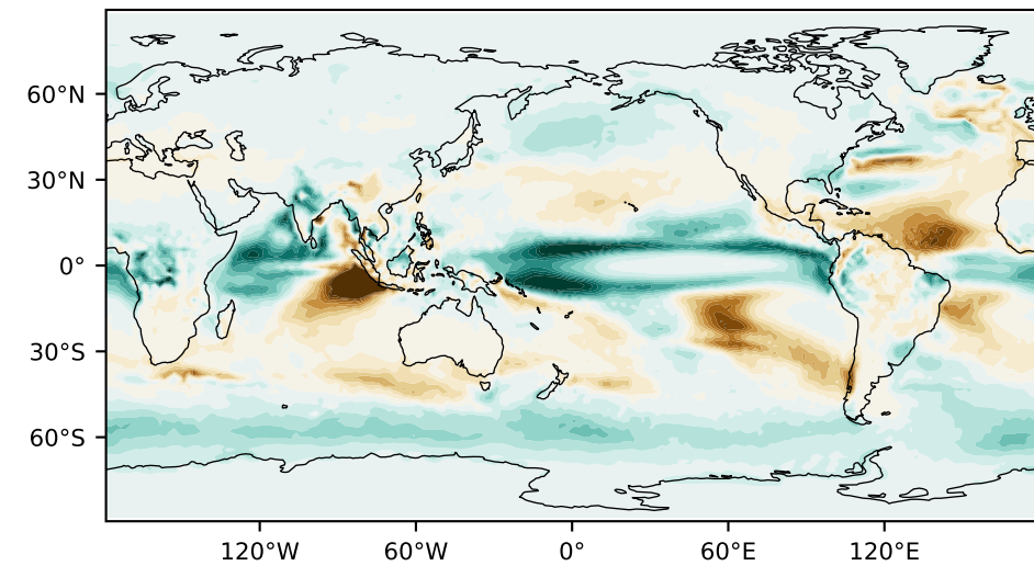
MRI-ESM2-0
