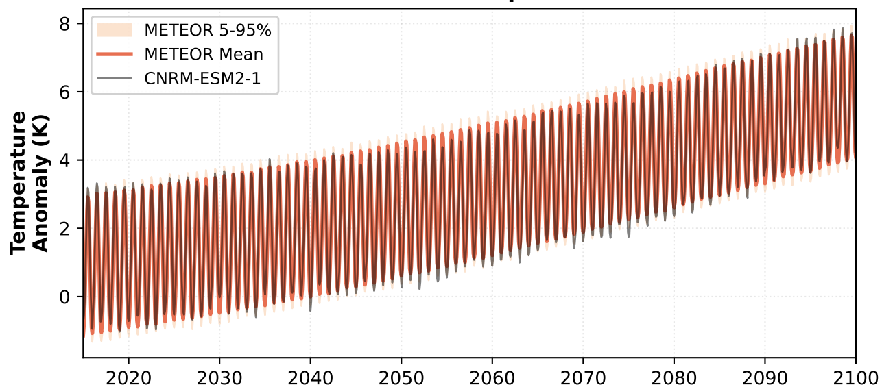
SSP5-3.4-OS - Temperature
