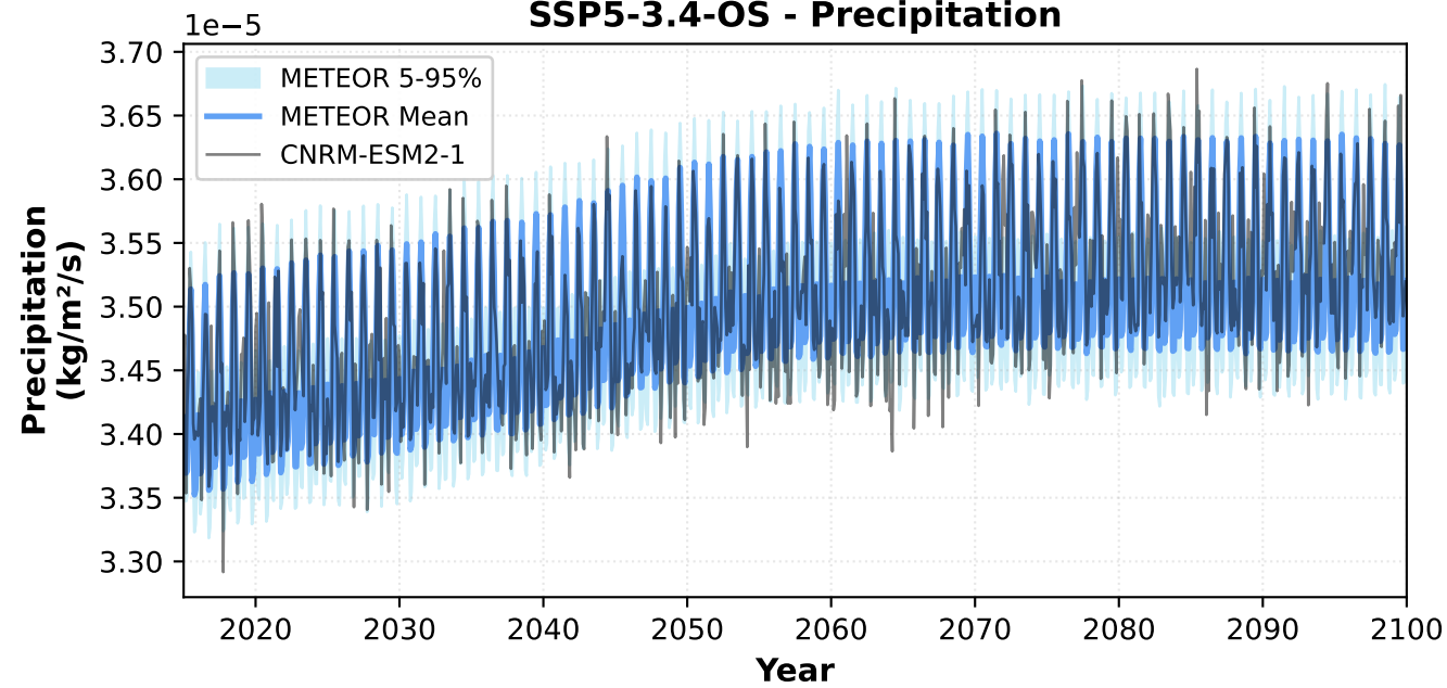
SSP5-3.4-OS - Precipitation
