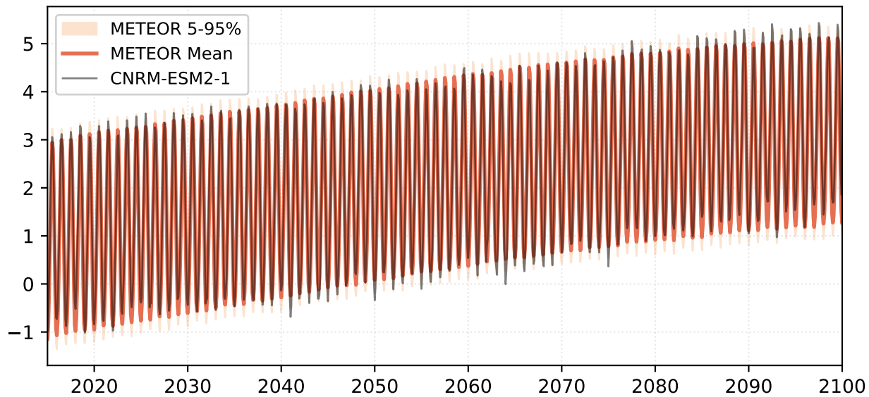
SSP5-8.5 - Temperature
