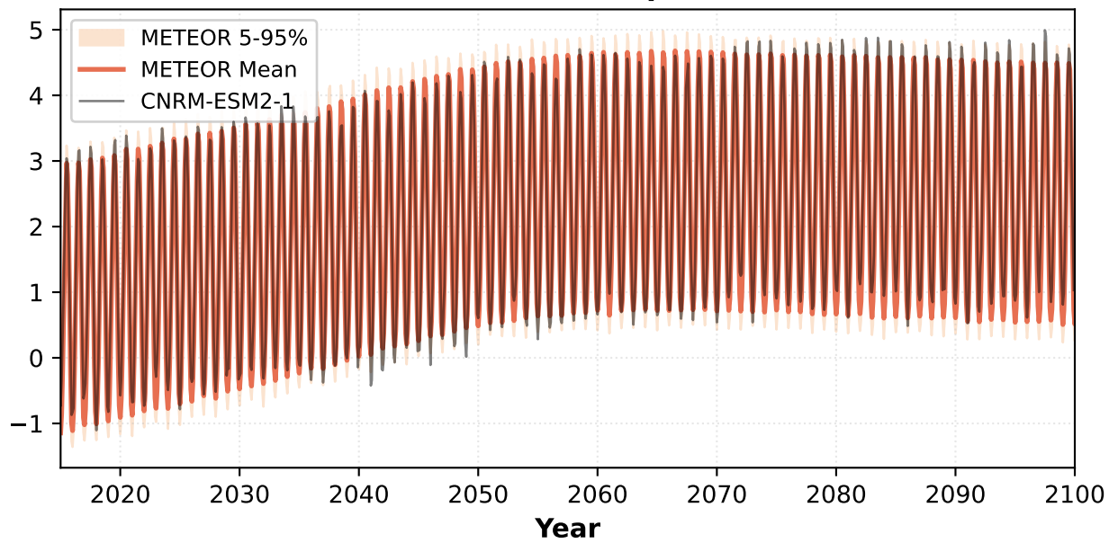
SSP5-3.4-OS - Temperature
