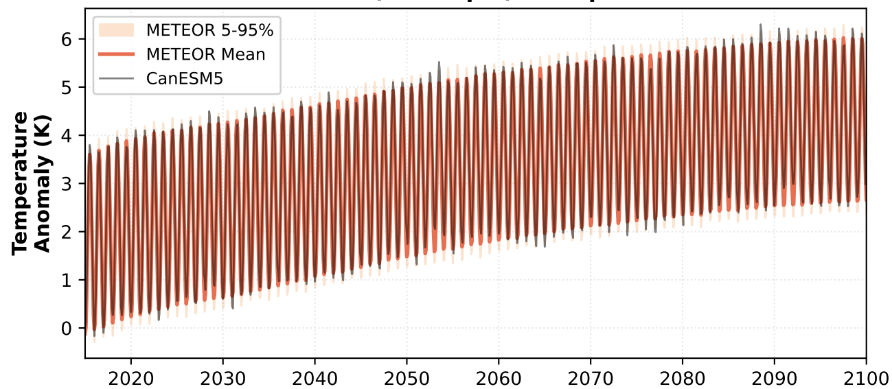
SSP5-8.5 - Temperature
