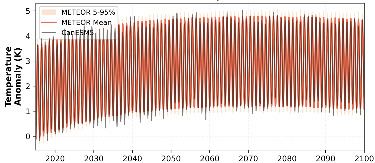
SSP2-4.5 (in-sample) - Temperature
