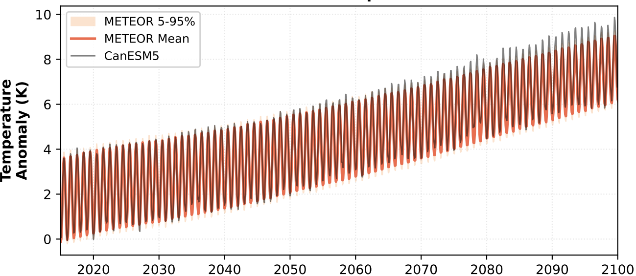
SSP5-3.4-OS - Temperature
