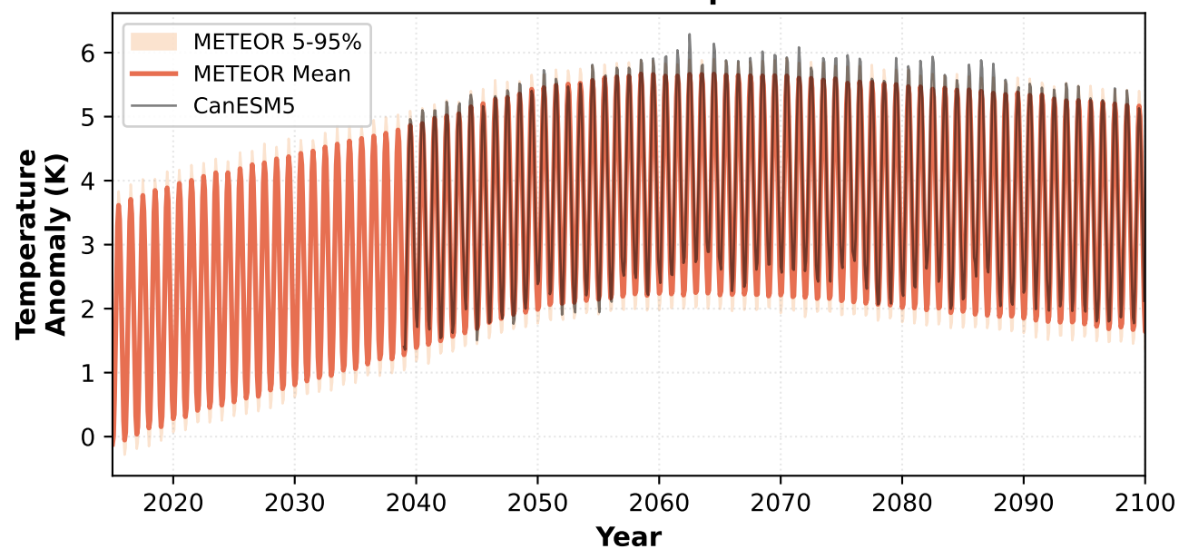
SSP5-3.4-OS - Temperature
