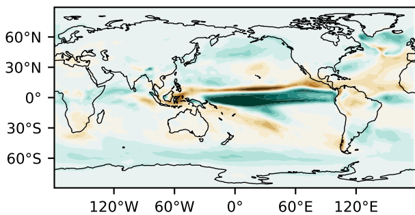
a METEOR
