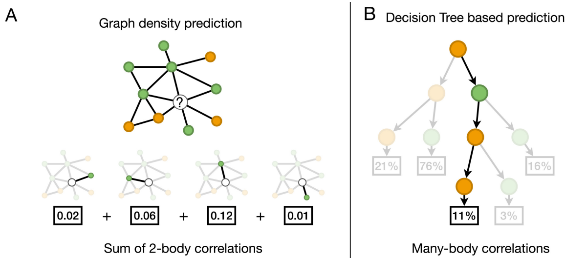
Figure 4.1: Node correlation: Density vs ML approach
