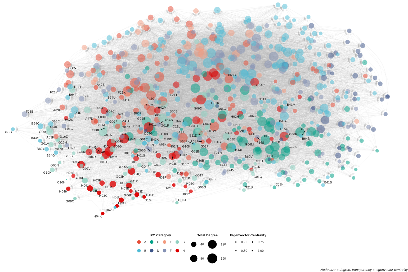
Figure 3.2: FITS Technology Network (based on 2018 patent data)
