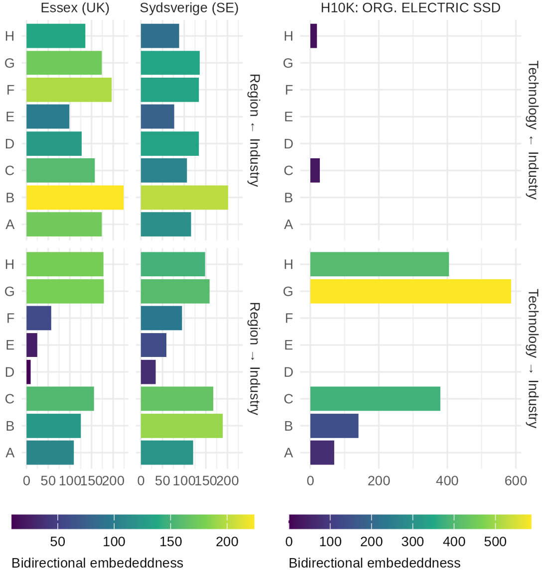
Figure 3.5: Bidirectional Embeddedness: profile of a region vs a technology
