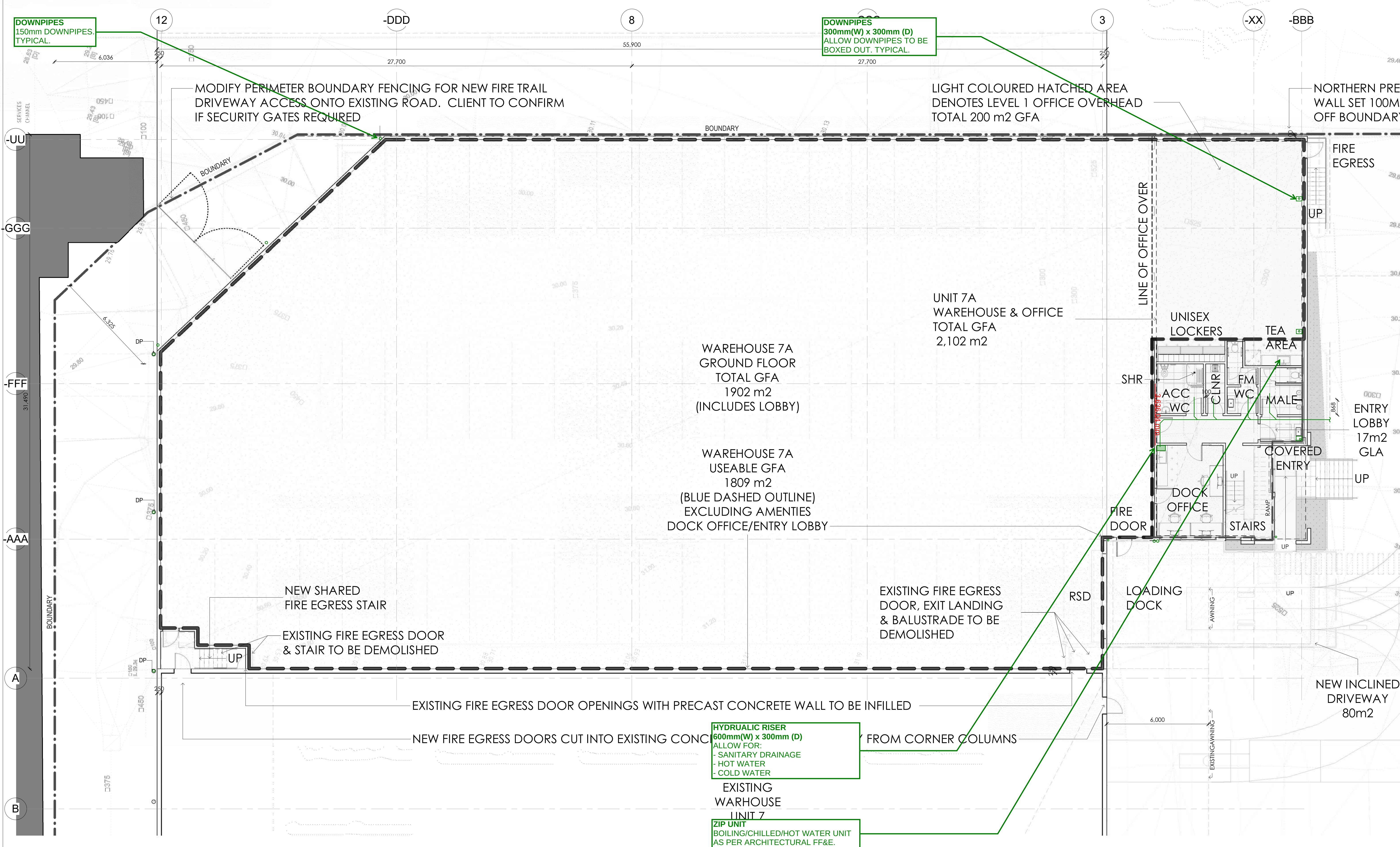
1 UNIT 7A - GROUND FLOOR PLAN 1 : 100 CD-600
