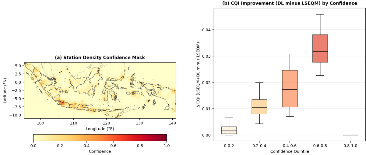
Figure 11: (a) Station density confidence mask C(x, y) , ranging from 0 (no station coverage) to 1 (saturated coverage, \geq 2 stations per 0.5^\circ cell). Gaussian smoothing ( \sigma = 1 grid cell) prevents sharp boundaries. (b) Relationship between confidence mask value and CQI improvement (LSEQM+DL minus LSEQM): box plots binned by confidence quintile.
