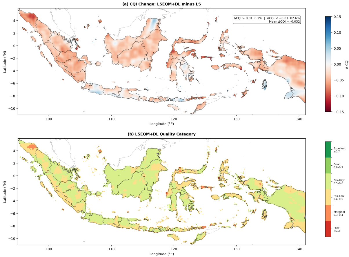
Figure 7: (a) Smoothed CQI difference map showing the mean difference between LSEQM+DL and LS across all 36 dekadal periods (positive values indicate improvement; Gaussian smoothing with \sigma = 1.5 pixels applied for visual clarity). (b) Six-tier quality classification of LSEQM+DL: Excellent ( \geq 0.7 , dark green), Good (0.6–0.7, green), Fair-High (0.5–0.6, yellow-green), Fair-Low (0.4–0.5, yellow), Marginal (0.3–0.4, orange), and Poor ( < 0.3 , red).
