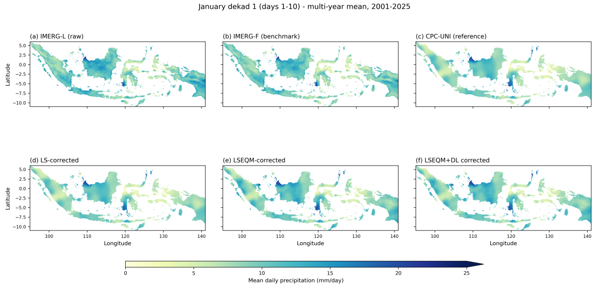
Figure 5: Climatological mean daily precipitation (mm/day) for January dekad 1 (days 1–10), averaged over 2001–2025: (a) IMERG-L (raw satellite product to be corrected), (b) IMERG-F (gauge-adjusted satellite benchmark), (c) CPC-UNI (gauge-based reference at 0.5^\circ , regridded to 0.1^\circ ), (d) LS-corrected, (e) LSEQM-corrected, (f) LSEQM+DL corrected. All panels use a common color scale; ocean cells are masked. The progression from (a) to (f) visualizes the framework’s effect on spatial precipitation patterns over the Indonesian archipelago.
