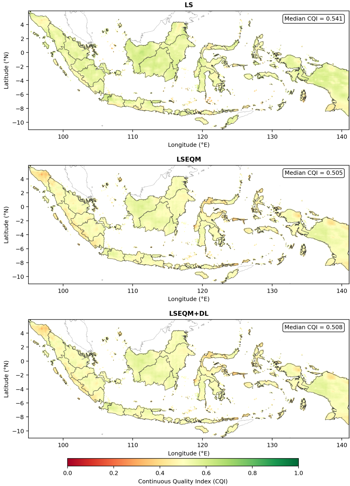
Figure 6: Spatial distribution of the Continuous Quality Index (CQI) for (a) Linear Scaling, (b) LSEQM, and (c) LSEQM+DL, evaluated against CPC-UNI. Values represent the mean CQI across all 36 dekadal periods. Higher values indicate better agreement with the reference dataset. The color scale ranges from 0 (poor) to 1 (excellent).
