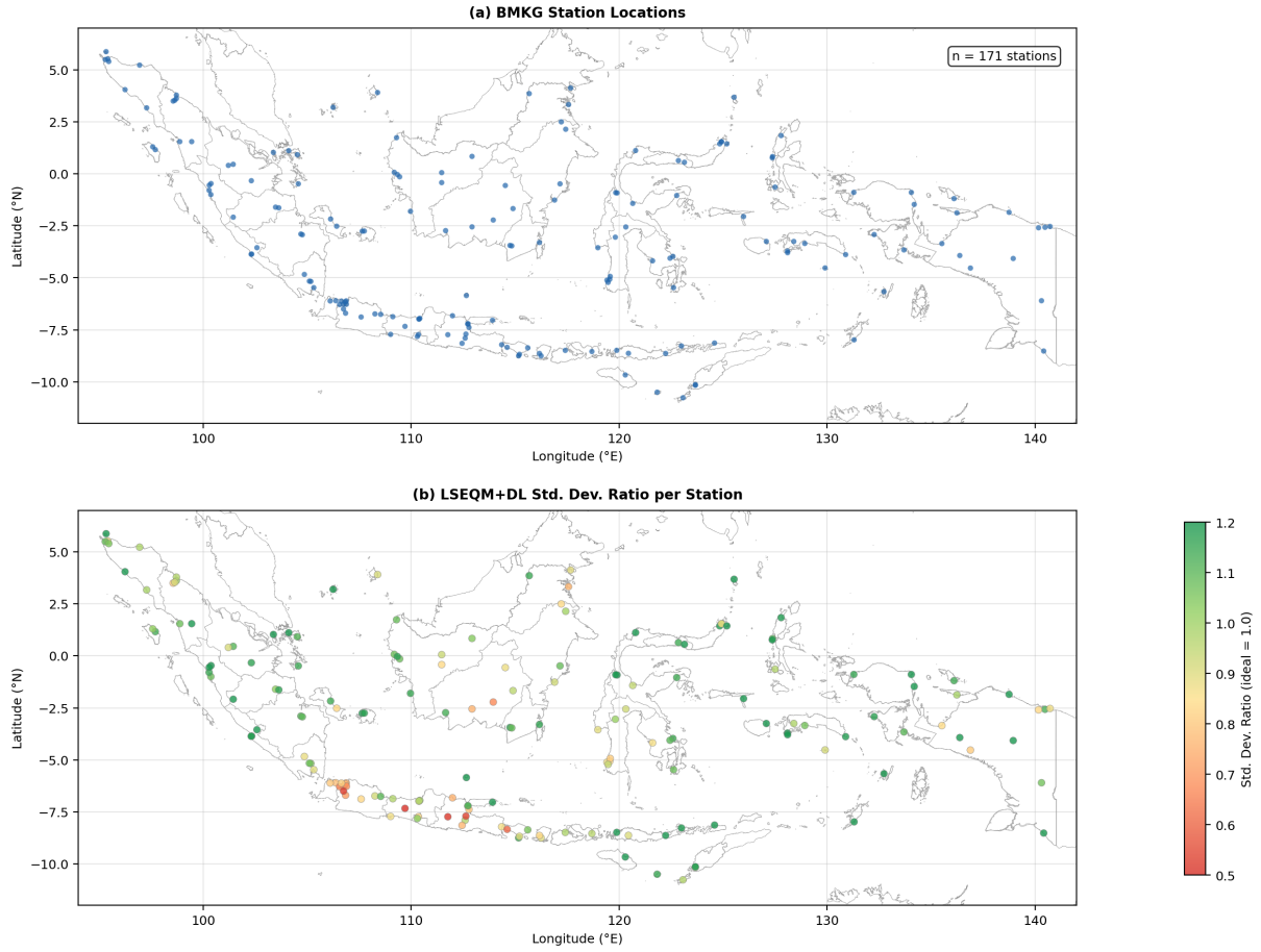
Figure 9: (a) Location of BMKG weather stations used for independent validation ( n = 171 ). (b) Per-station standard deviation ratio (test/observed) for the LSEQM+DL product, averaged across all dekadal periods. Values near 1.0 (green) indicate good variability preservation; values below 0.7 (red) indicate underestimation of observed variability.
