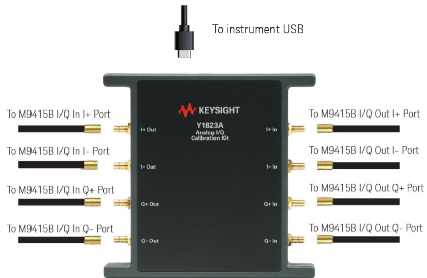
Figure 1. Y1823A Calibration kit for Analog baseband I/Q
