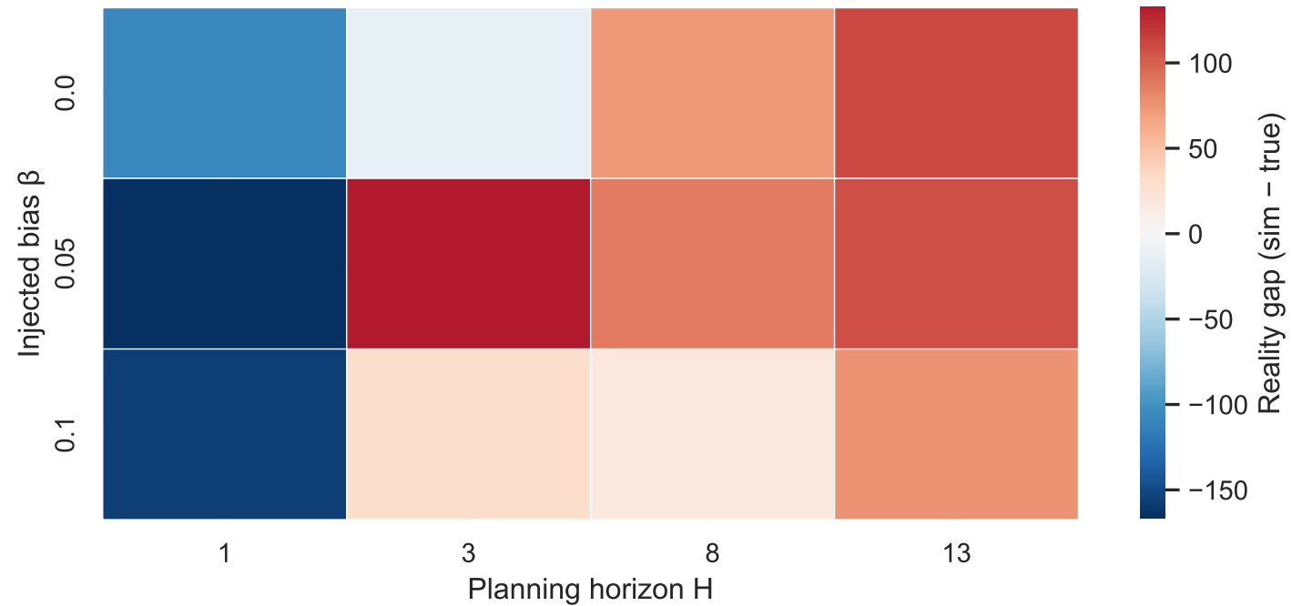
Confounded regime: reality gap heatmap ( \gamma=0.95 )
