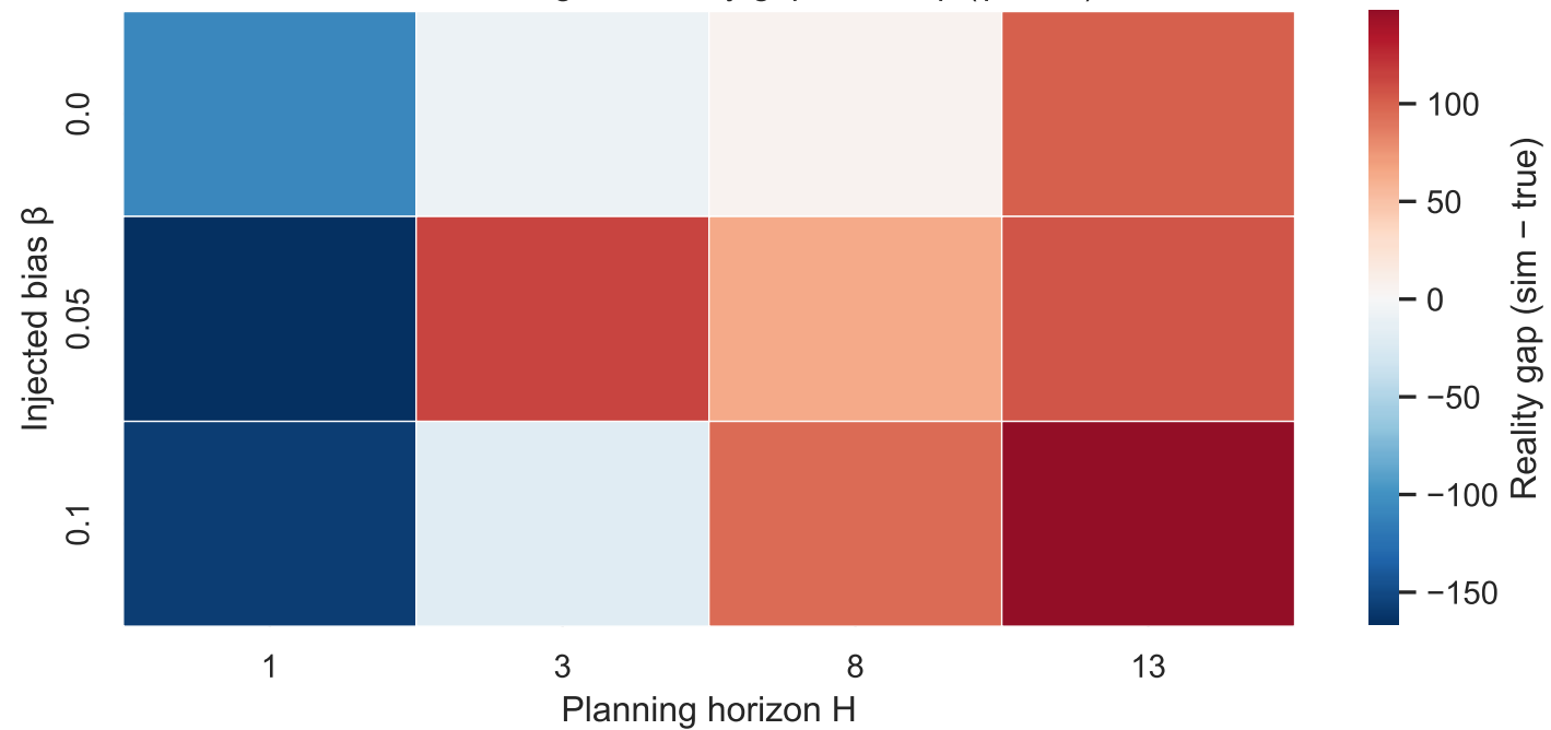
Confounded regime: reality gap heatmap ( \gamma=0.99 )
